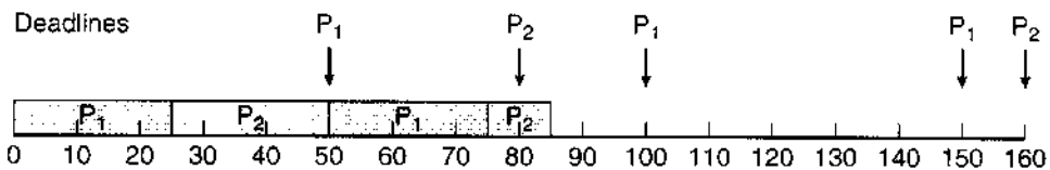
Figure 19.9 Missing deadlines with rate-monotonic scheduling.
