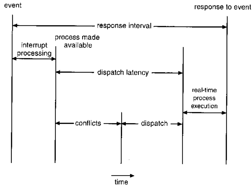
Figure 19.5 Dispatch latency.
