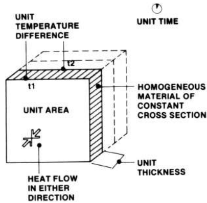
Fig. 11. Conductivity
