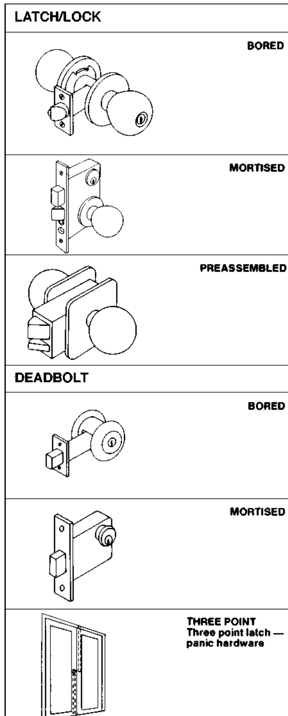
Fig. 3. Door lock types and uses (Source: Sweet's Catalog File Selection Data 1993 by permission of McGraw-Hill)
