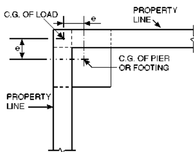
Fig. 11. Eccentric corner footing plan. Note: eccentricities are removed by walls acting as pumphanhandles. Each wall removes the eccentricity normal to it.
