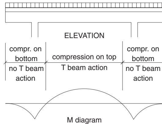
Fig 10. T beam
