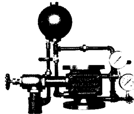
Fig. 5. Alarm valve
