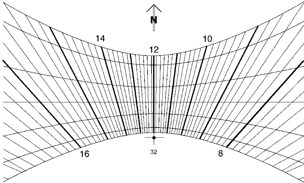
Fig. 27. Gnomonic sun-path diagram for LAT = 32°
