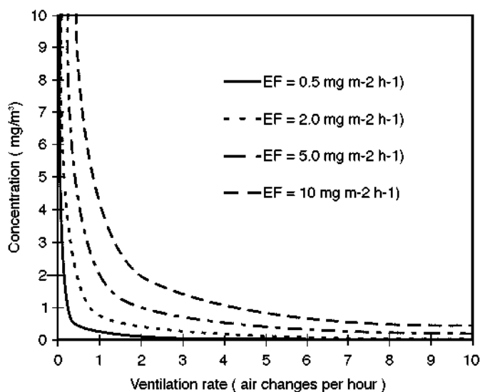
Fig. 5. Contaminant concentration as a function of source strength and air exchange rate.
