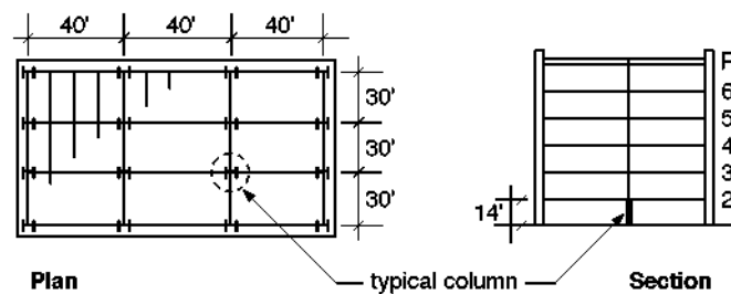
Fig. 9. Typical column in steel framed building
