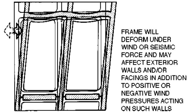
LATERAL DISPLACEMENT
