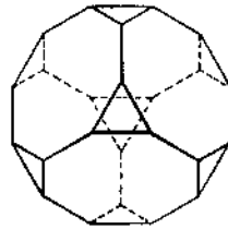
TRUNCATED CUBE F 3 F 6 V E 8 6 24 36
