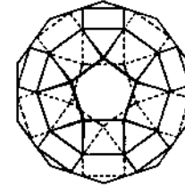
RHOMBICOSIDODECAHEDRON F 2 F 4 F 5 V E 20 30 12 60 120
