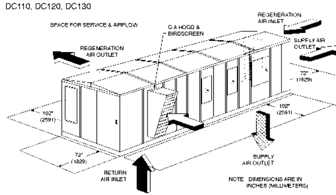
Fig. 3. Self-contained dessicant air conditioner (Source: Englehard/ICC)
