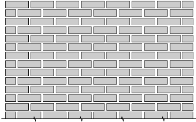
Fig. 2. Running bond
