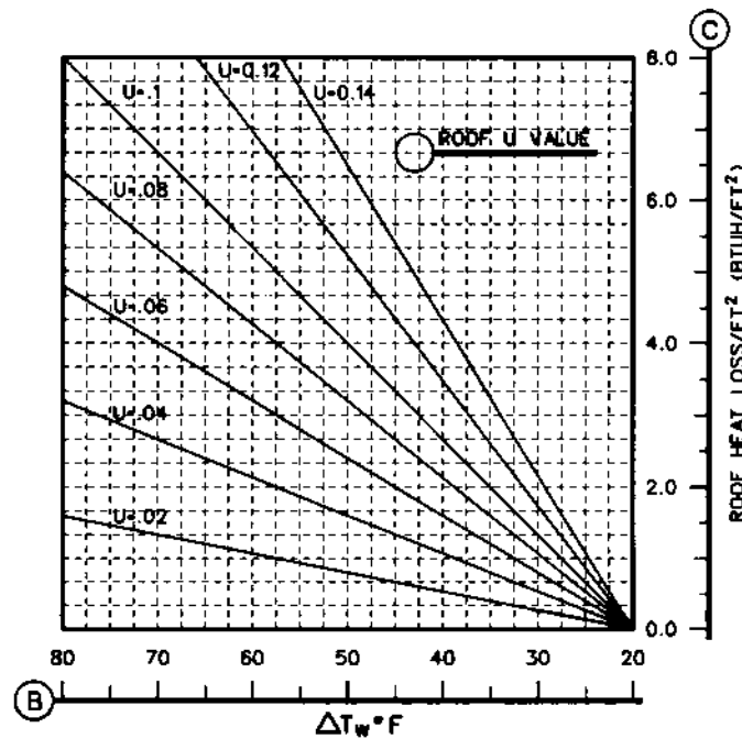
Nomograph 5
