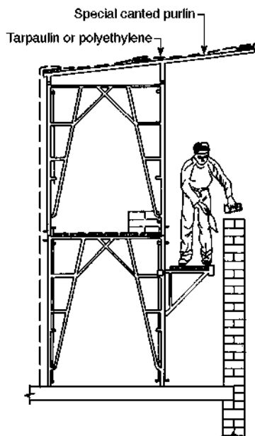
Fig. 52. Scaffold-type enclosure
