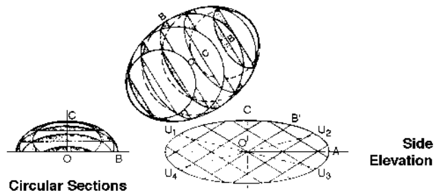
Circular Sections
