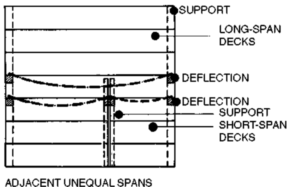
Fig. 11. Structural deformation in decks and girders
