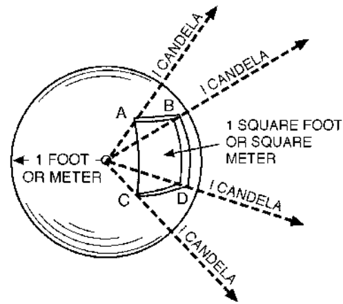
Fig. 3. Illustration of the relationship between intensity, luminous flux, and illuminance.
