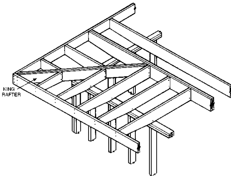
Fig. 11. Corner detail of flat roof with overhang of more than 3 ft.
