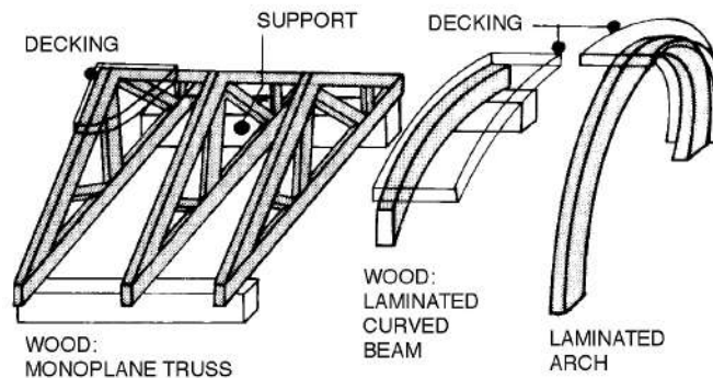
Fig. 25. Trusses/beams: pitched/curved
