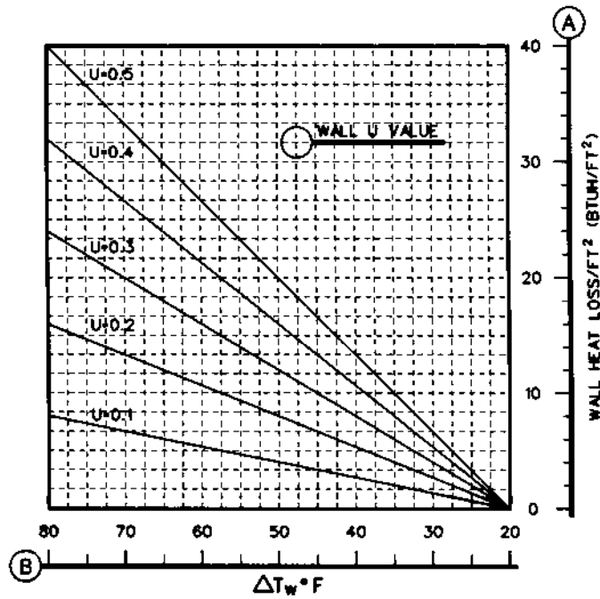
Nomograph 4
