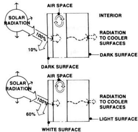
Fig. 2. Radiation: reflectivity
