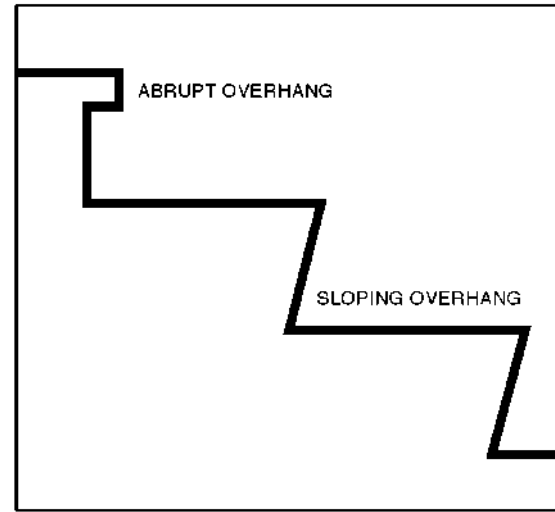
Fig. 6. Nosing overhangs
