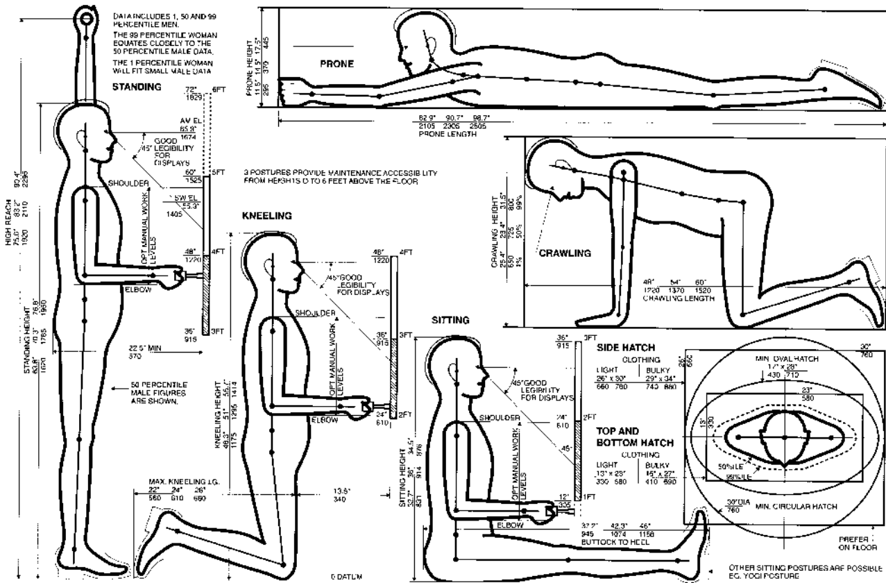
Fig. 4. Maintenance access (whole body).
