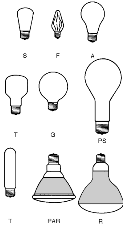
Fig. 7. Typical incandescent lamp shapes.
