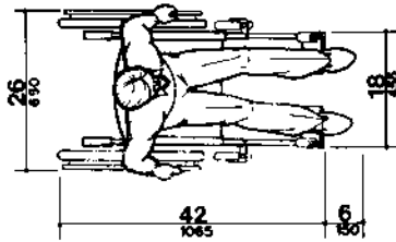
Wheelchair dimensions
