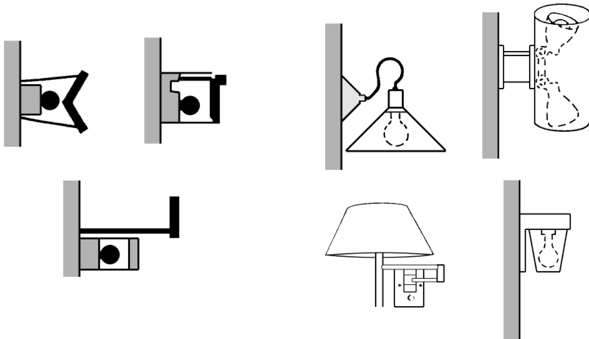
Fig. 14. Wall-mounted luminaires.
