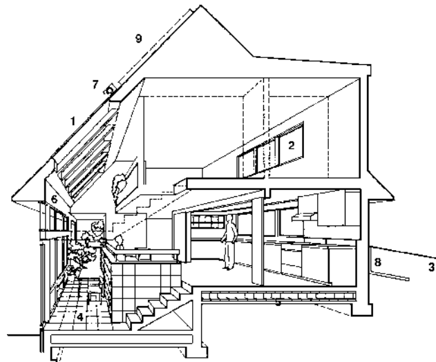
Fig. 4. Combination of passive solar, energy conservation and energy-efficient fuel system.
