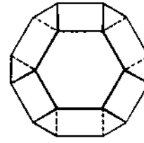
TRUNCATED OCTAHEDRON F 4 F 6 V E 6 8 24 36
