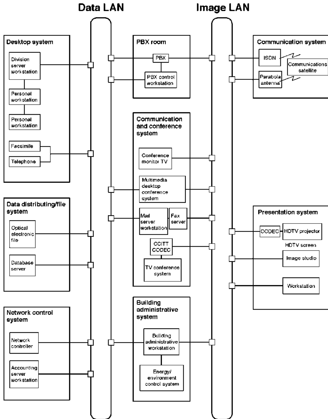
Fig. 3. A schematic diagram a local area network
