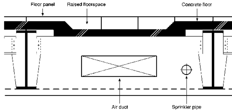
Fig. 2. Structural details of an access floor
