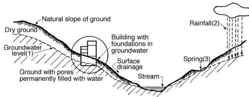
Fig 1. Basic Factors affecting groundwater level,
