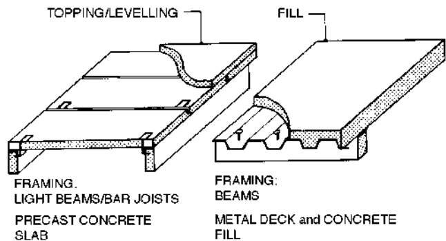
Fig. 17. Roof/floor: flat
