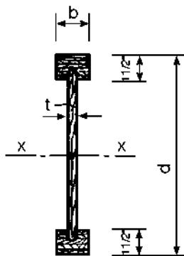
(k) Trus Joint
