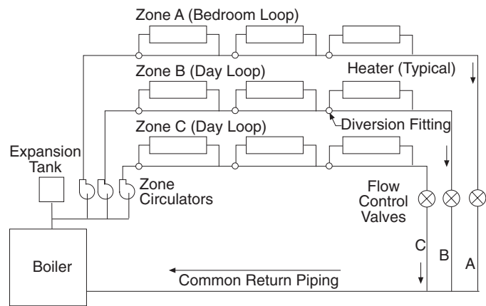
Fig. 10. Zoning of series loops
