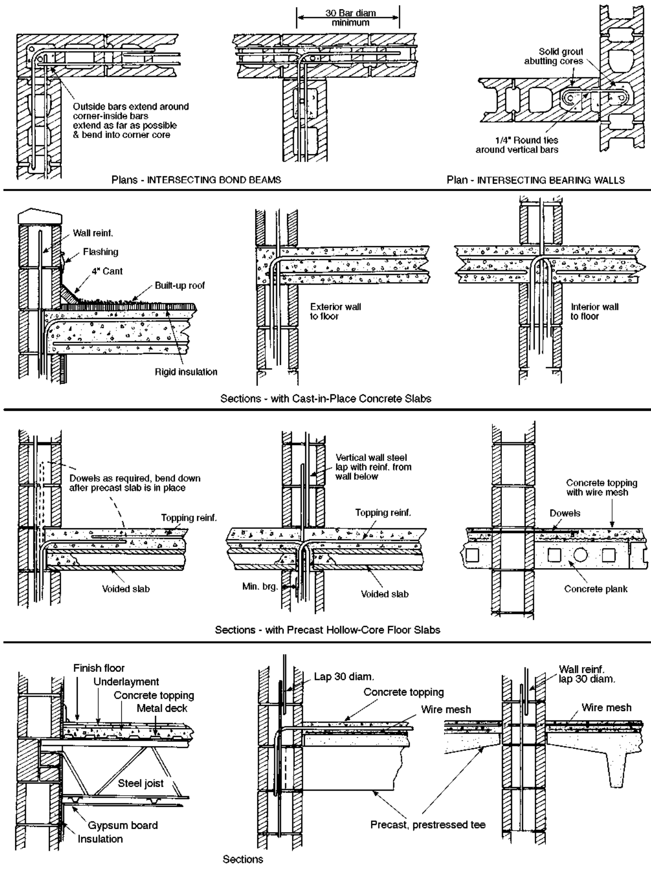
Fig. 40. Construction details, reinforced concrete masonry
