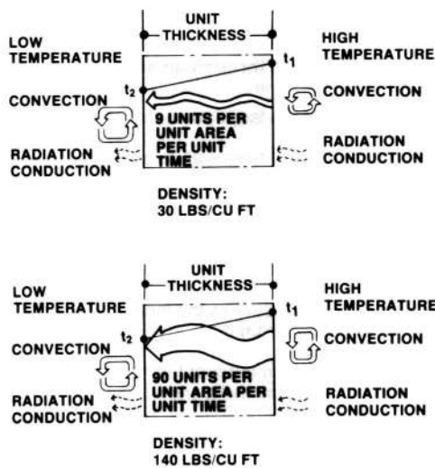
Fig. 7. Conduction
