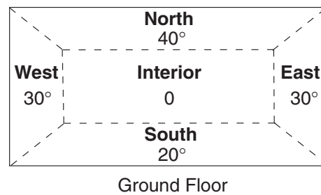
Fig. 3. Representative heating balance points for a two-story office building
