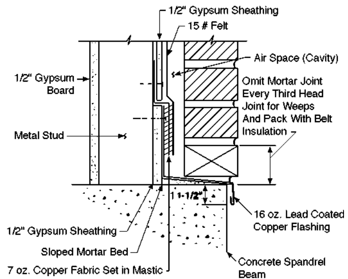
Fig. 2. Through-wall flashing of brick veneer/steel stud wall.
