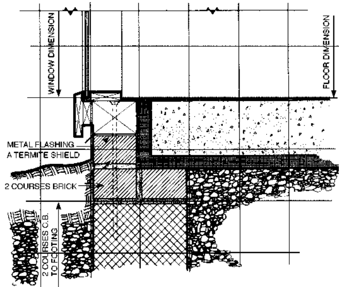
Fig. 12. Section and detail of frame building
