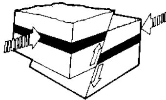
Fig. 1c. Thrust or reverse fault
