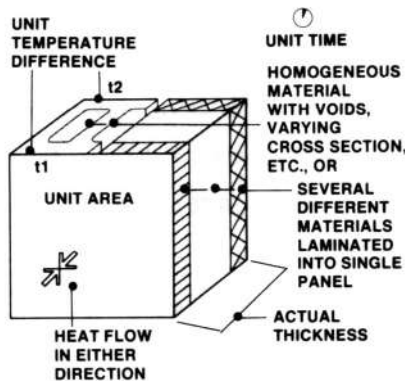
Fig. 12. Conductance
