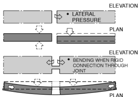
Fig. 3. Transverse movement
