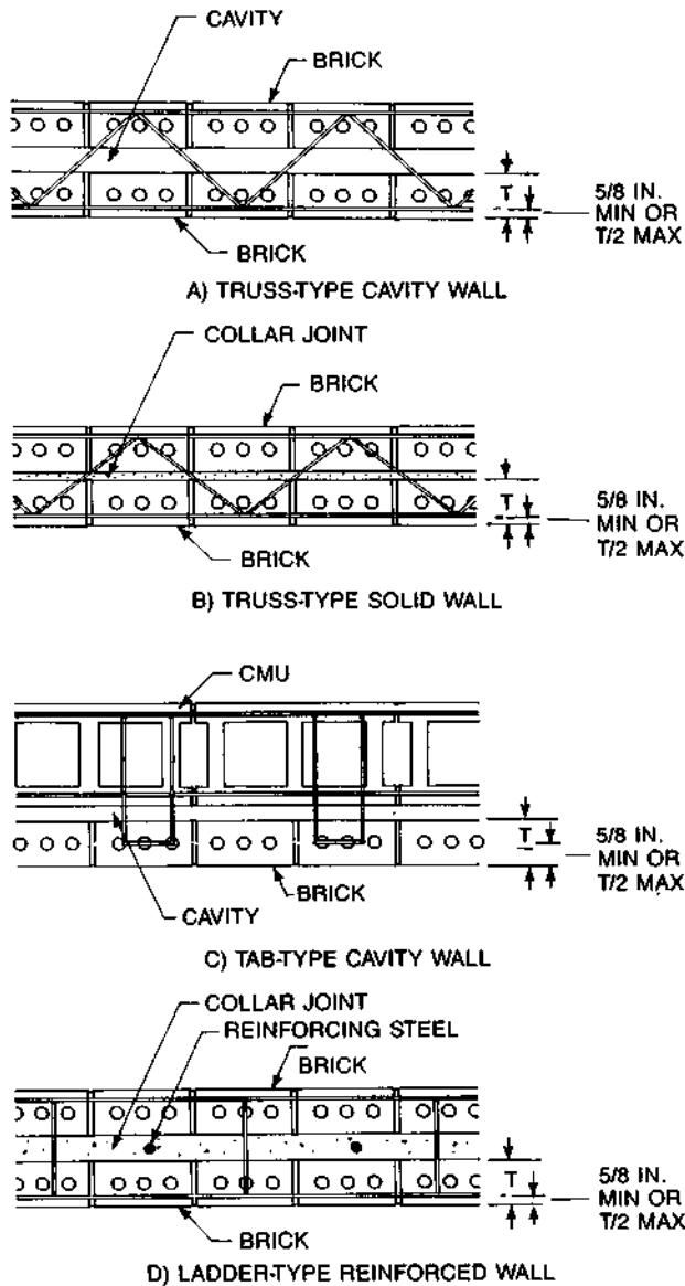
Fig. 9. Joint reinforcement details (Source: Brick Institute of America).
