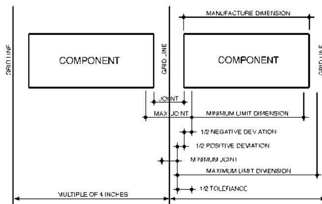
Fig. 1. Basis for sizing a component
