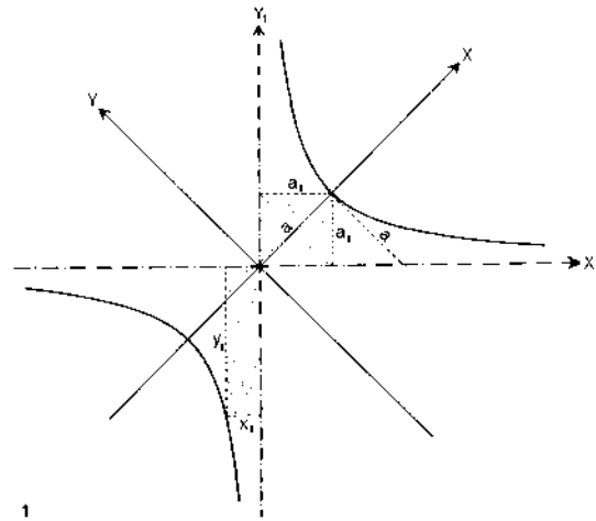
TWO CASES FOR HYPERBOLA
