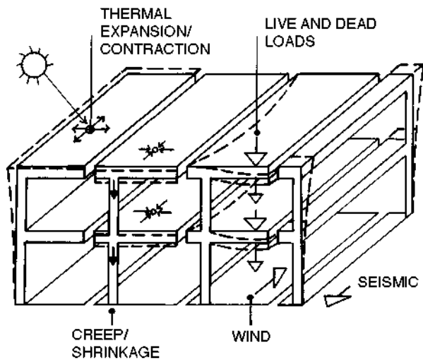
Fig. 10. Deformations defined
