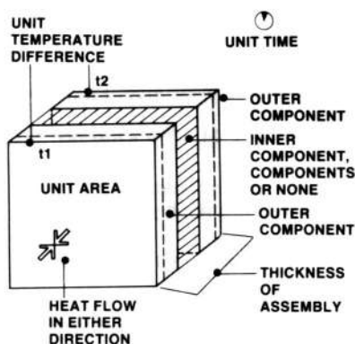
Fig. 13. Transmittance
