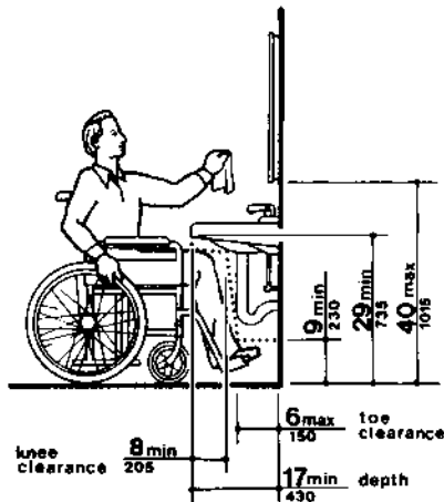
Lavatory clearances
