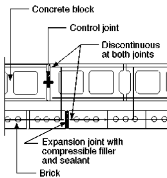
Fig. 31. Masonry control joint detail
