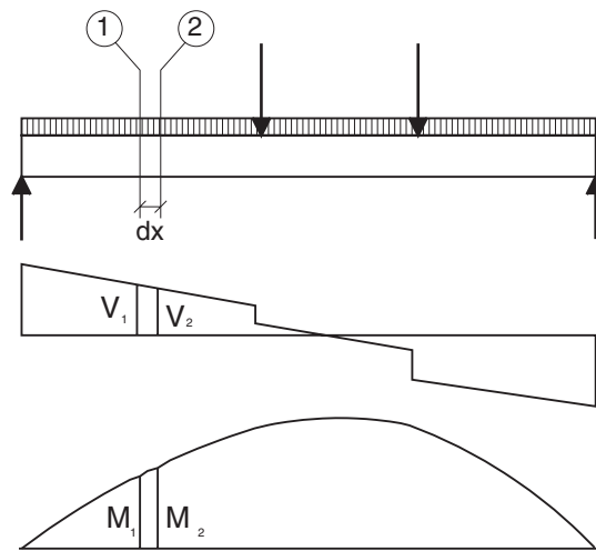
Fig. 13. Shear and moment diagram
