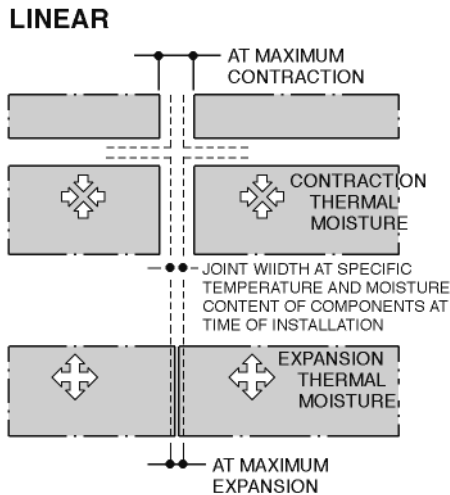
Fig. 1 Linear movement
