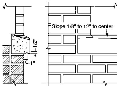
Fig. 49. Sill detail to prevent wash
