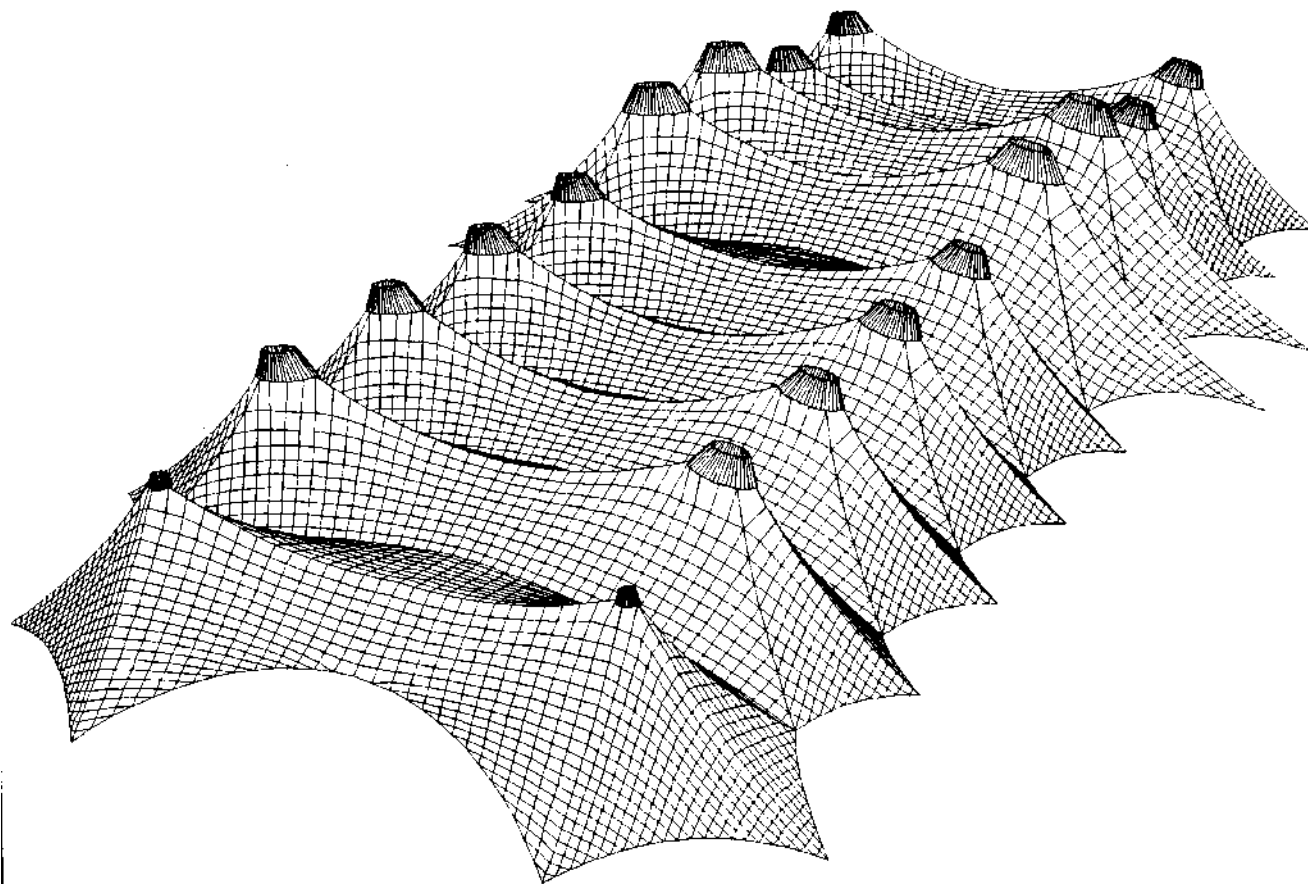
Fig. 3. Geodesic net analysis of the Denver Airport Terminal Building (Berger 1996).
