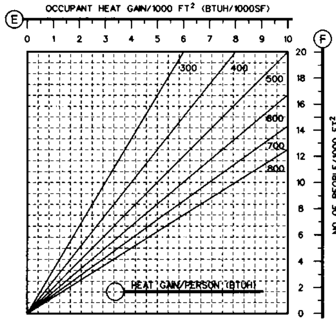
Nomograph 7
