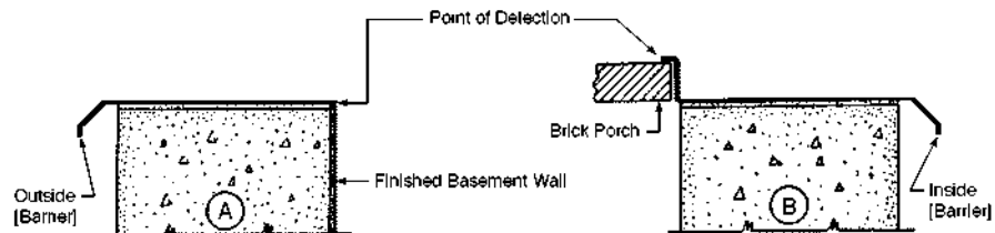
Fig. 3. Deflector shield
