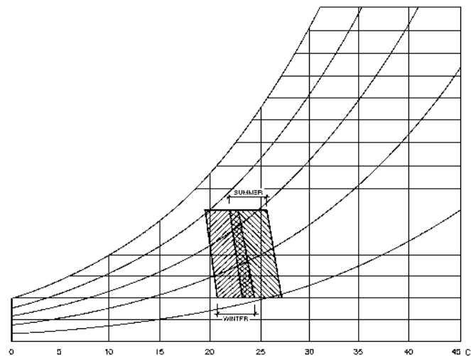
Fig. 6. Comfort zone defined by the ASHRAE Comfort Standard
