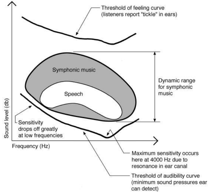
Fig. 3. Human audible sound level and frequency (Egan 1988)
