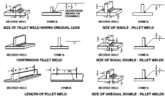
Fig. 22. Use of welding symbols
