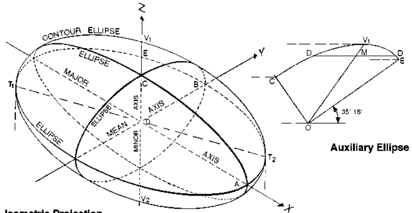
Isometric Projection
