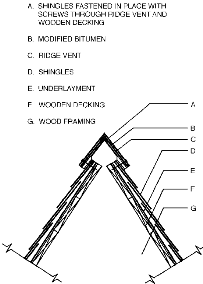
Fig. 2. Ridge with vent.
