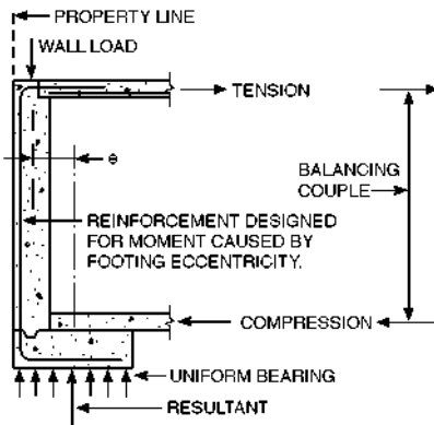
Fig. 10. Eccentric wall footing section
