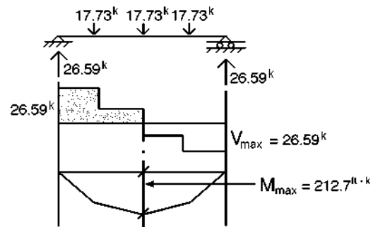
Fig. 13. Load, shear and moment diagrams
