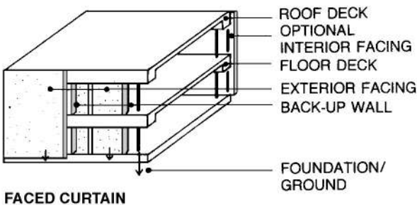
Fig. 5. Wall elements
