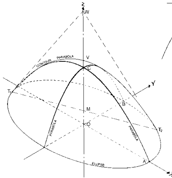
Isometric Projection
