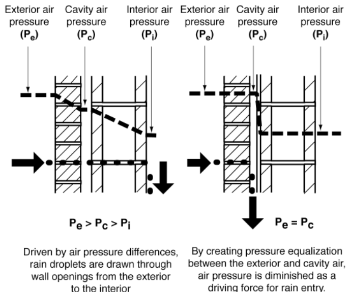
Fig. 5. Air Pressure Difference as a Driving Force for Rain Entry
