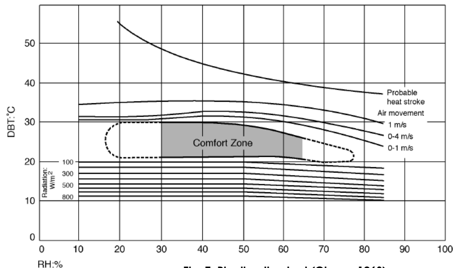
Fig. 7. Bioclimatic chart (Olgay 1963)
