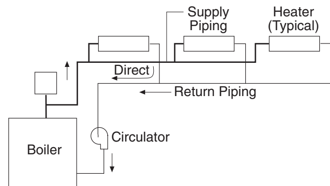
Fig. 11. Two-pipe direct return piping arrangement
