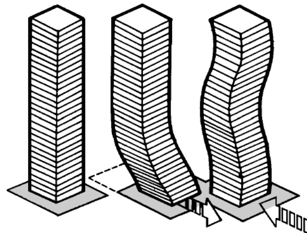
Fig. 6. Effects of cyclic reversals on ground acceleration. At the same time that the upper part of the structure begins to move to catch up with the initial displacement, the ground motion reverses itself.
