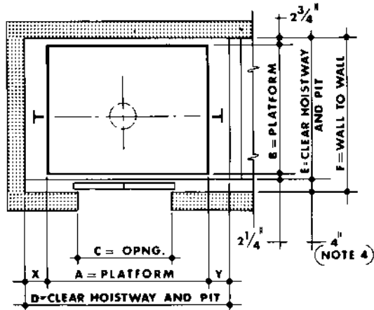
PASSENGER ELEVATOR
