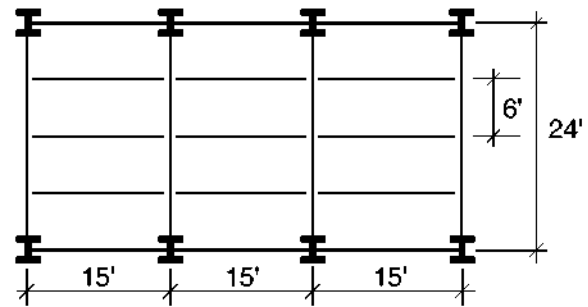
Fig. 11. Framing plan
