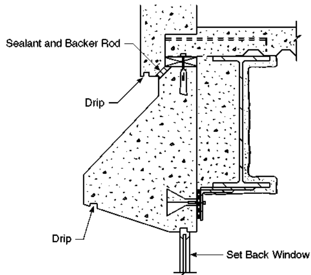
Fig. 3. Vertical section showing horizontal joinery in precast concrete panels. Note ship-lap geometry and recessed sealant to shield the joint from the weather.
