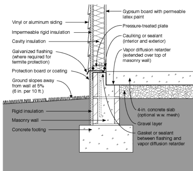
Fig. 7. Slab-on-grade foundation with exterior insulation. Note: This detail is suitable for a mixed (temperate) or overheated (warm) climate. Source: Lstiburek and Carmody (1993)—revised 1997.
