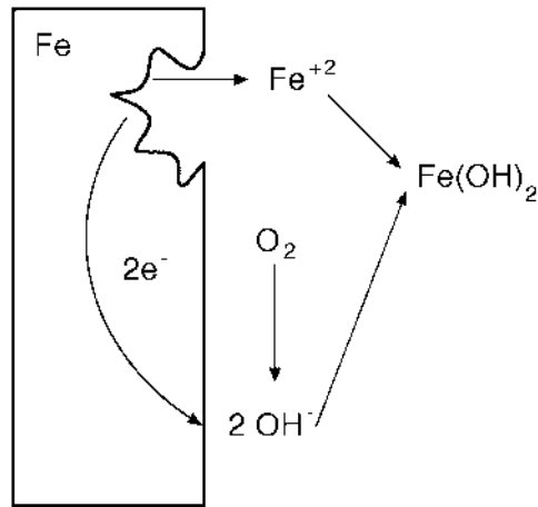
Fig. 2. Iron in aerated environment, neutral or basic
