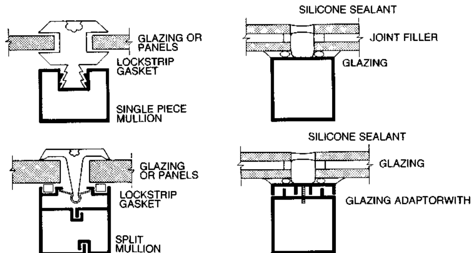
Fig. 10. Curtain wall mullion types.
