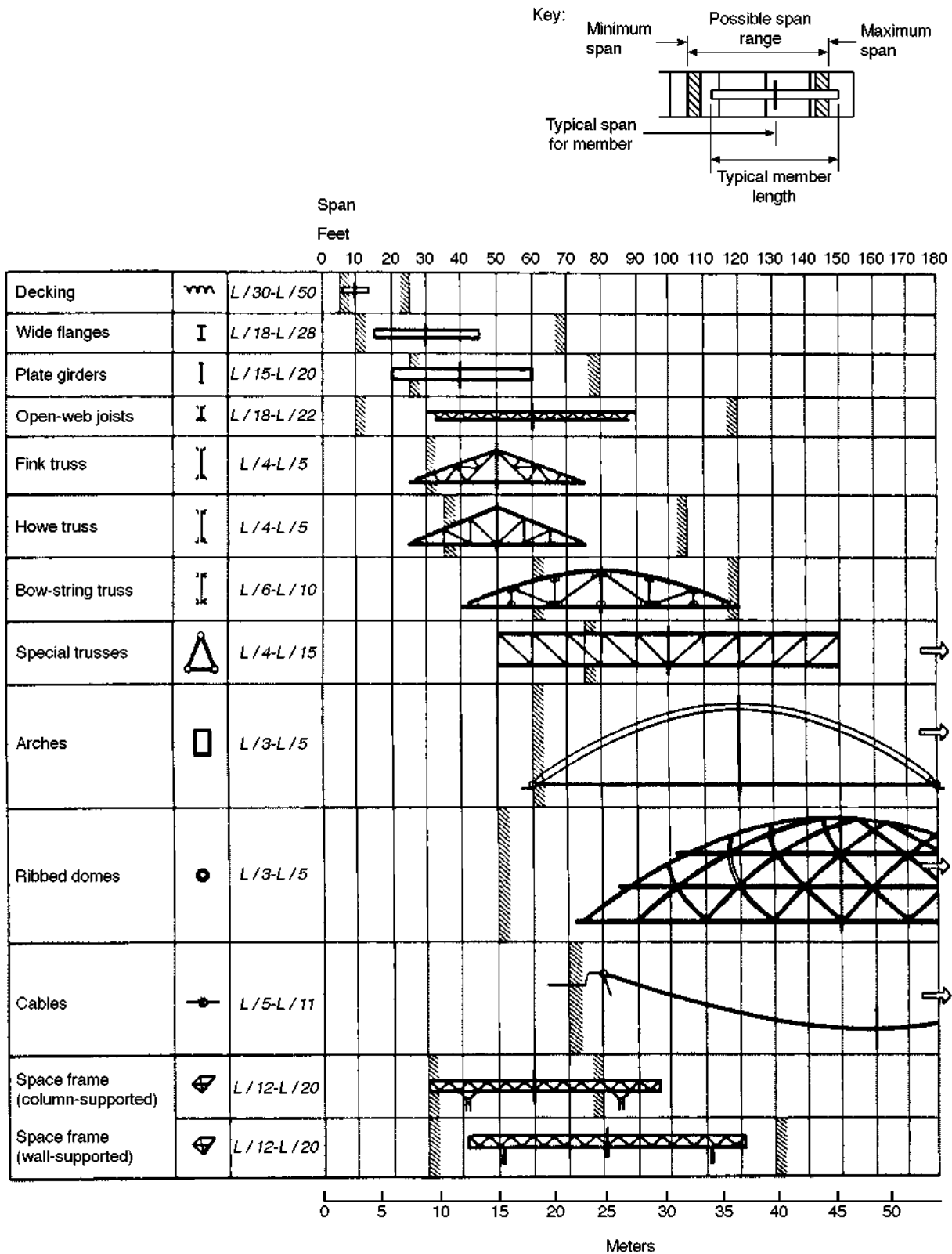
Fig. 27. Aproximate span ranges for steel systems. Source: Schodek (1992). Reproduced by permission of Prentice Hall.
