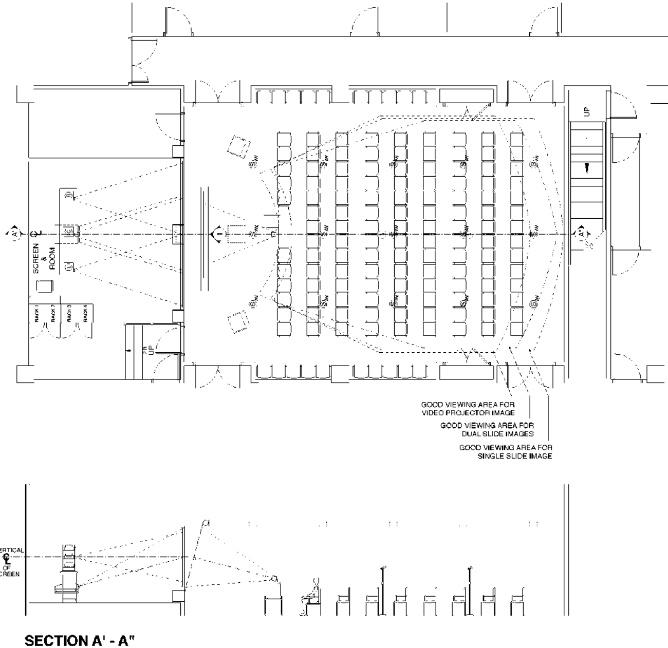
Fig. 1. Audiovisual facilities plan and section
