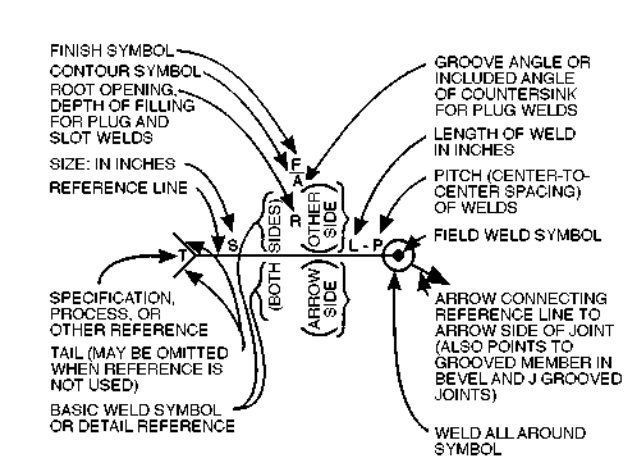
Fig. 21. Standard welding symbols
