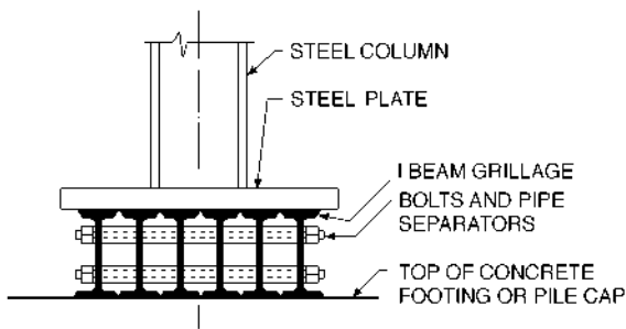
Fig. 3. Steel grillage
