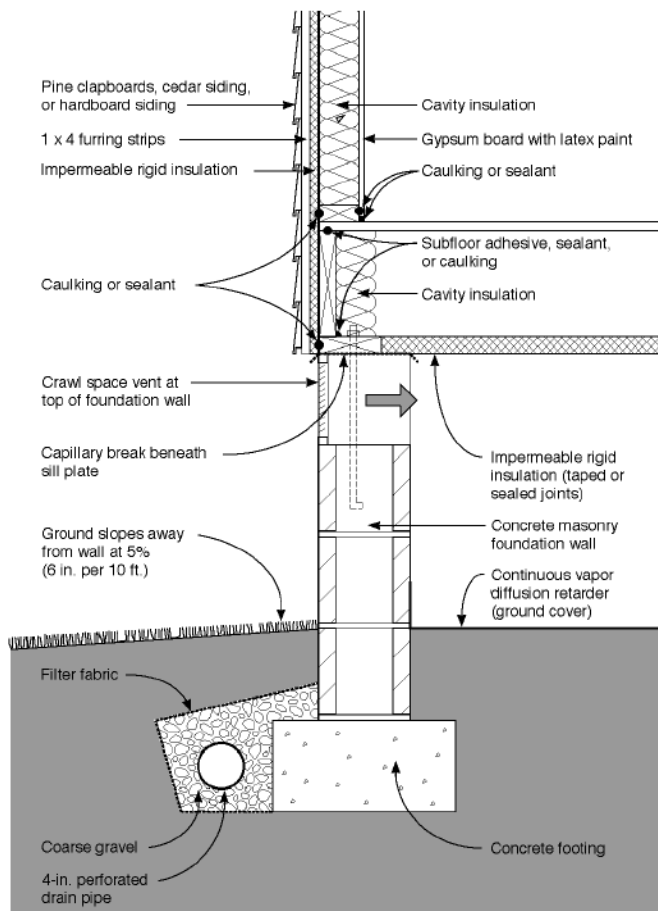
Fig. 4. Vented crawl space. Note: This detail is suitable for a mixed (temperate) climate. Source: Lstiburek and Carmody (1993)—revised 1997.
