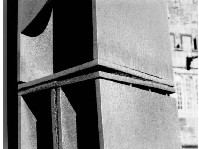
Fig. 7. Corrosion between bolted steel plates.
