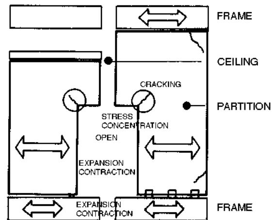
Fig. 13. Deformation effects on partitions
