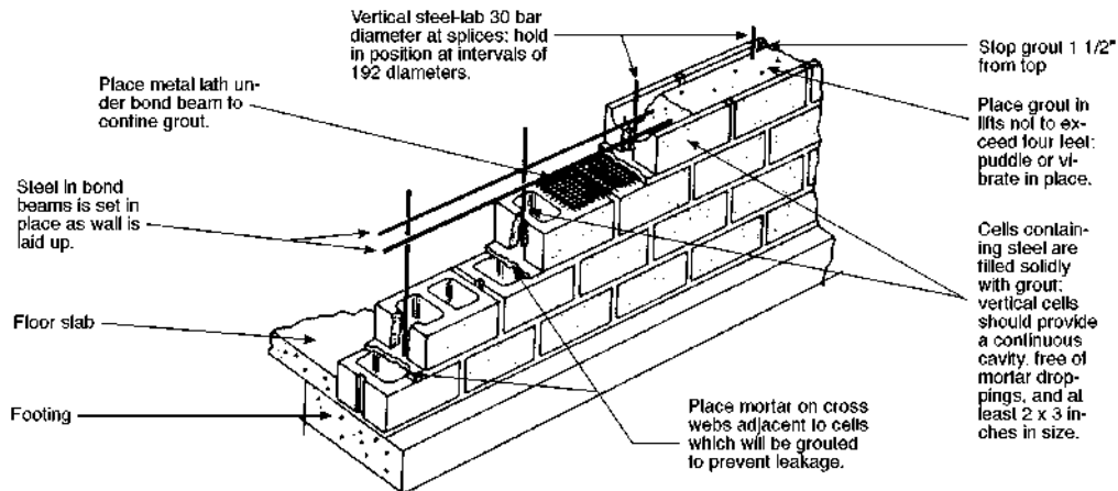
Fig. 37. Typical reinforced concrete masonry construction
