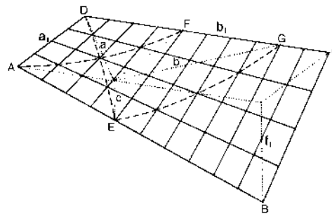
Axonometric projection
