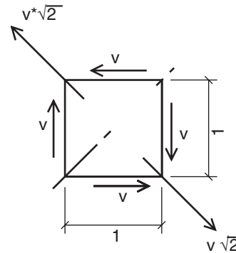
Fig. 16. Shear forces on isolated concrete cube
