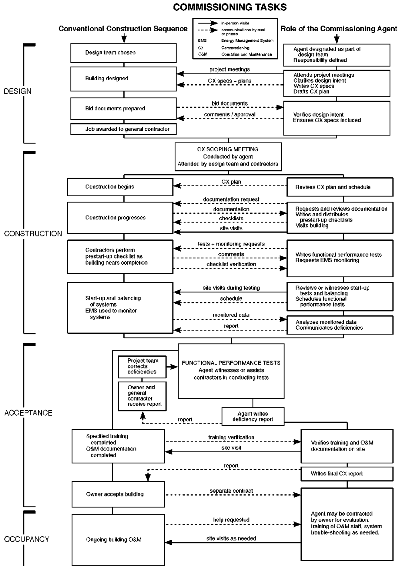
Fig. 3. Commissioning tasks (after ASHRAE 1995)
