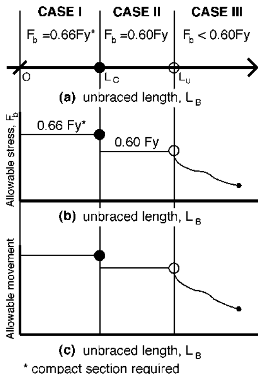
Fig. 10. Unbraced length of beams: relationship to (a) L_c and L_u ; (b) allowable stress; and (c) allowable moment
