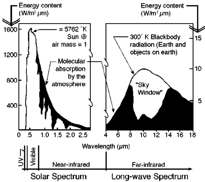
Fig. 1. Solar (short-wave) and thermal (long-wave) spectrum
