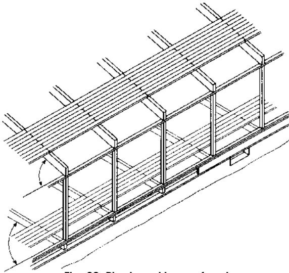
Fig. 20. Plank and beam framing
