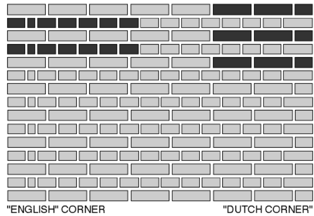
Fig. 6. English bond
