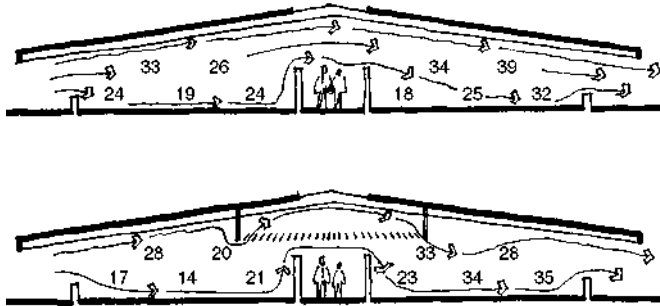
MIAMI, OKLAHOMA Fig. 16. Comparison of air flow across a classroom building created by modifications of ceiling geometry
