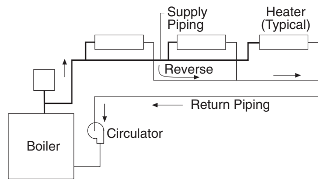
Fig. 12. Two-pipe reverse return piping
