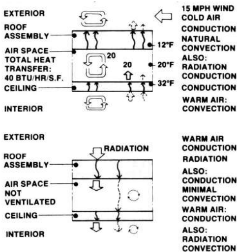
Fig. 6. Convection and radiation: horizontal air space
