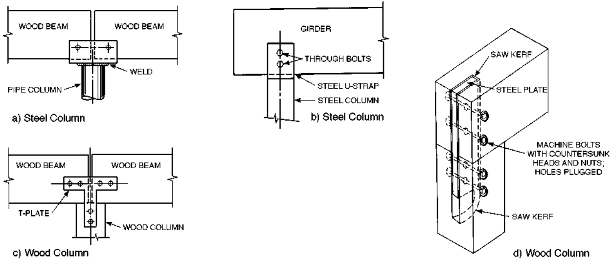
Fig. 30. Beam to column connections
