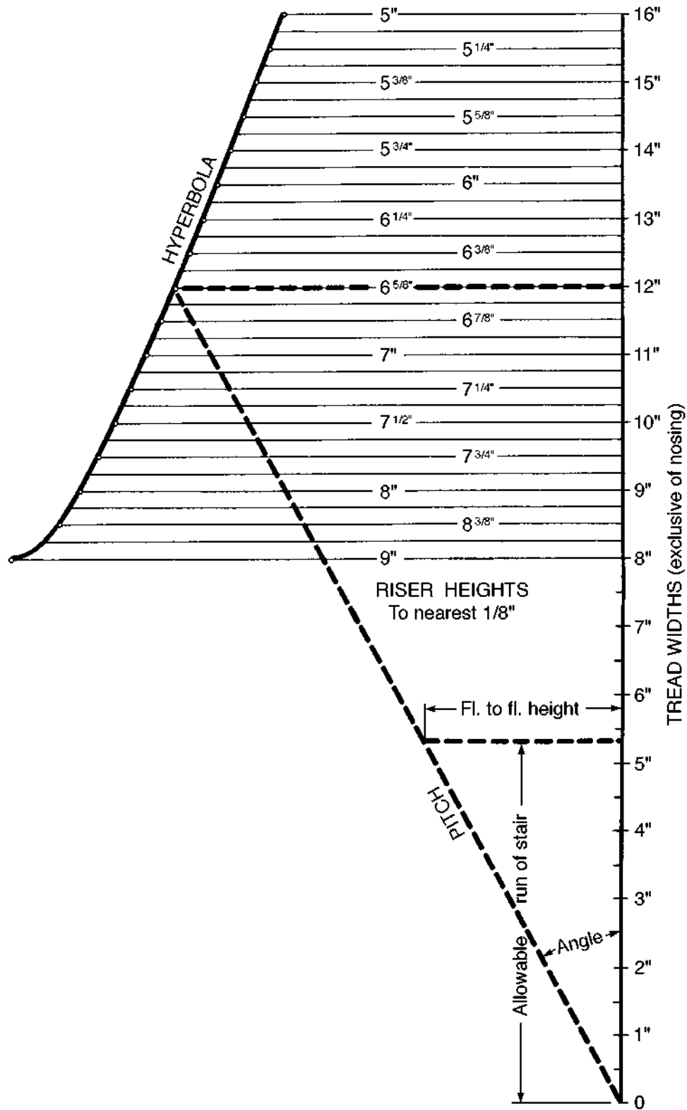
Fig 1. Proportional tread and riser nomograph All dimensions are 1/2 full size Metric conversion factor: 1 inch = 25.4 mm = 2.54 cm
