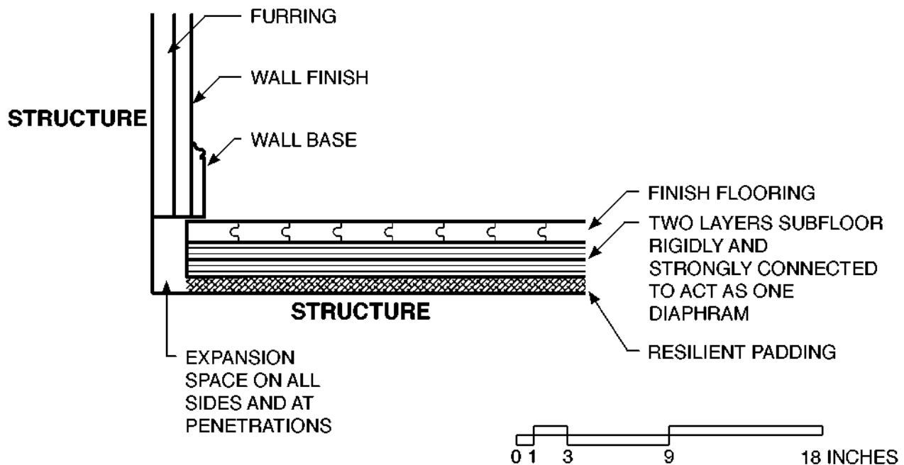
Fig. 9. Floating wood floor
