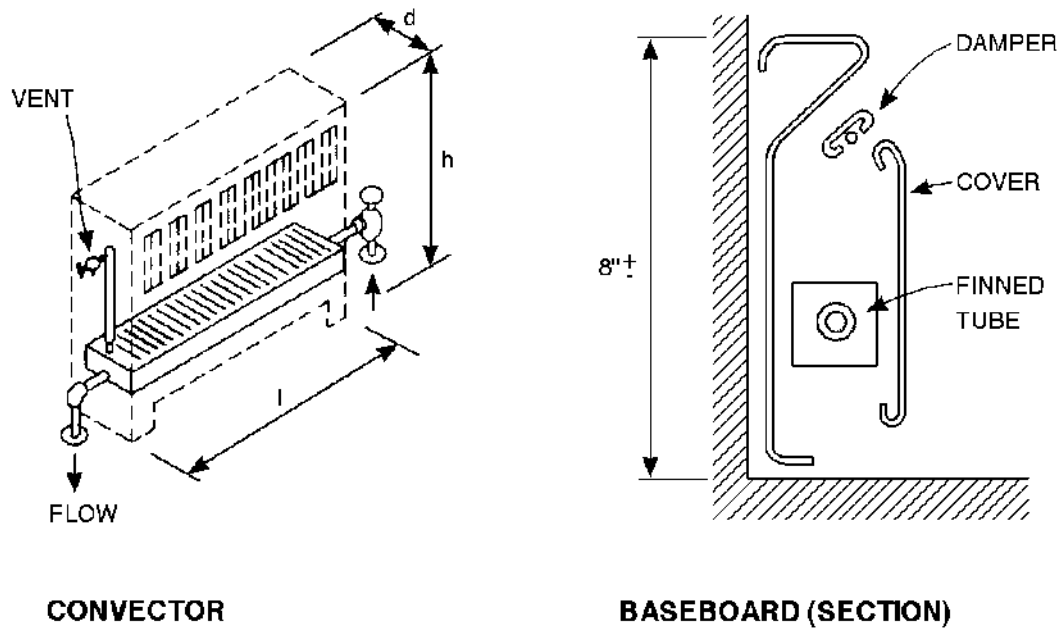
Fig. 14. Terminal heating devices in hot water systems
