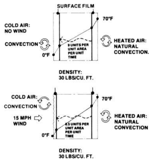
Fig. 4. Convection: surface conductance
