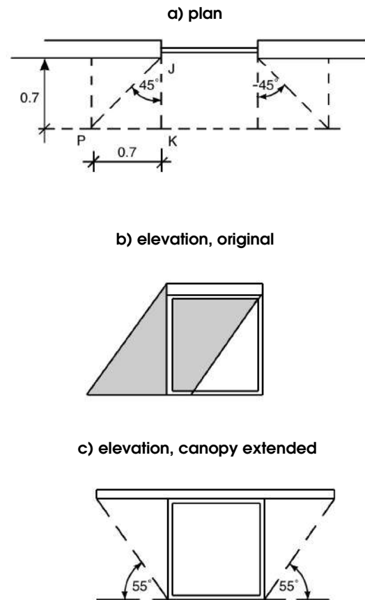
Fig. 50. Sideways extension of canopy:
