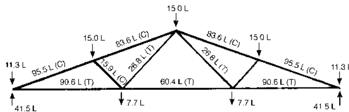
External and Internal Forces (lbs.) in Terms of Truss Span L (ft.)
