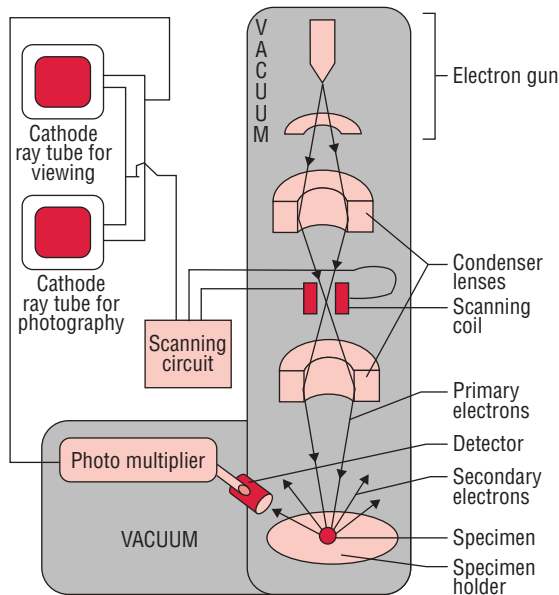
FIG. 2-5. Principle of electron microscopy.
