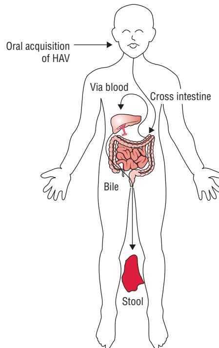
FIG. 66-2. Pathogenesis of hepatitis A virus infection.
