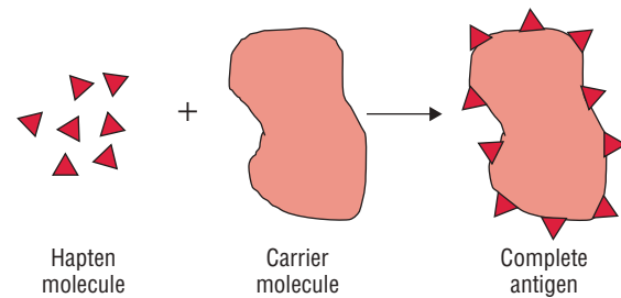
FIG. 12-1. Hapten-carrier conjugate.
