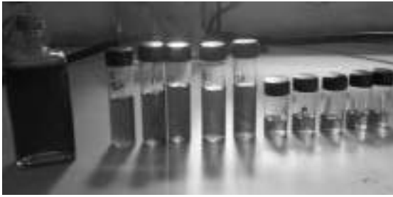
FIG. 76-1. Eijkman test.
