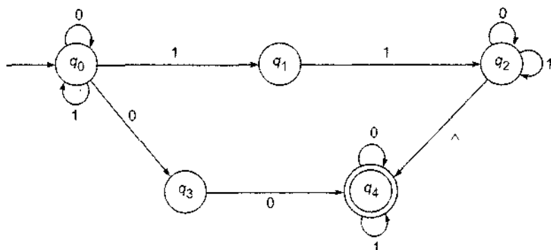
Fig. 3.8 Transition system for a nondeterministic automaton.
