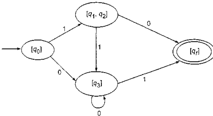
Fig. 5.22 Reduced DFA of Example 5.14.
