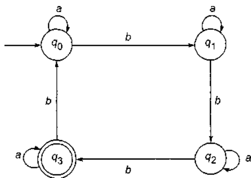
Fig. 5.35 DFA for Example 5.35.
