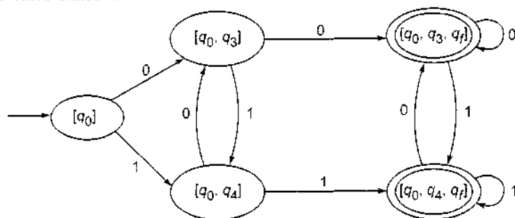
Fig. 5.19 Finite automaton of Example 5.13.
