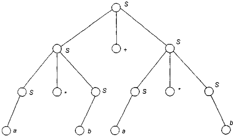
Fig. A6.1 Derivation tree for Exercise 6.1.
