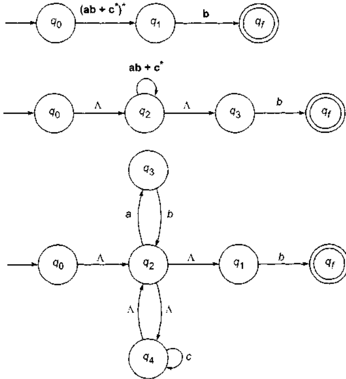
Fig. A5.3 Transition system for Exercise 5.9.
