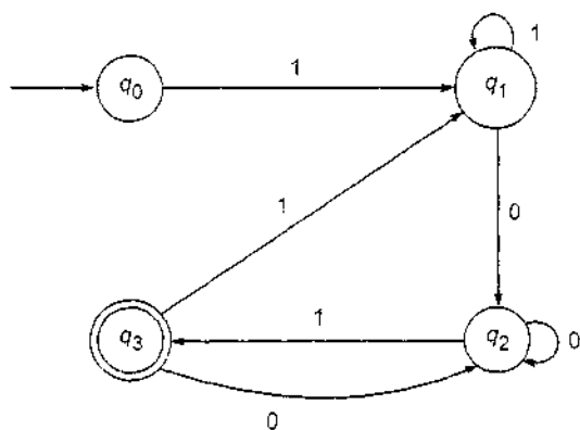
Fig. 5.38 Transition system of Exercise 5.8.
