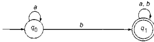
Fig. 5.32 DFA of Example 5.24, without \Lambda -moves.
