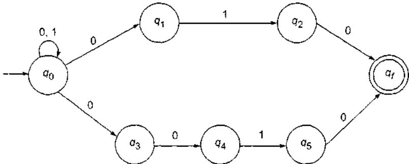
Fig. A5.4 N DFA for Exercise 5.12.
