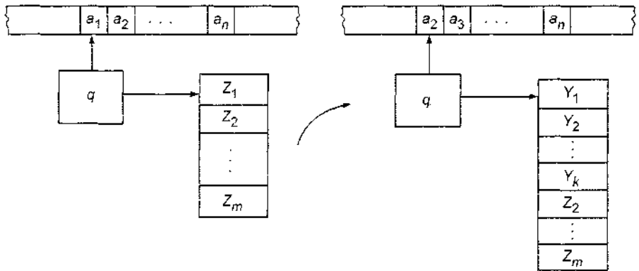
Fig. 7.2 An illustration of the move relation.
