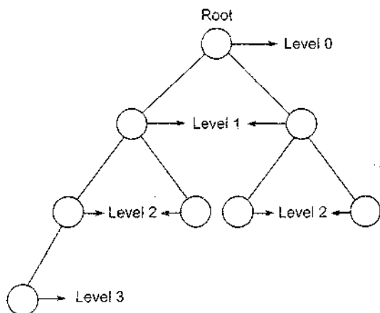
Fig. 2.10 Illustration of levels of vertices.
