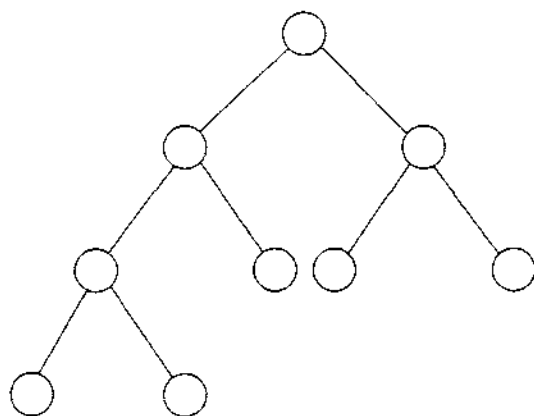
Fig. 2.11 Binary tree of minimum height with 9 vertices.
