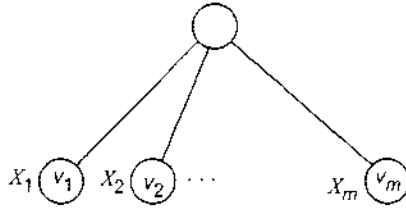
Fig. 6.6 Derivation tree with yield X_1 X_2 \dots X_m .
