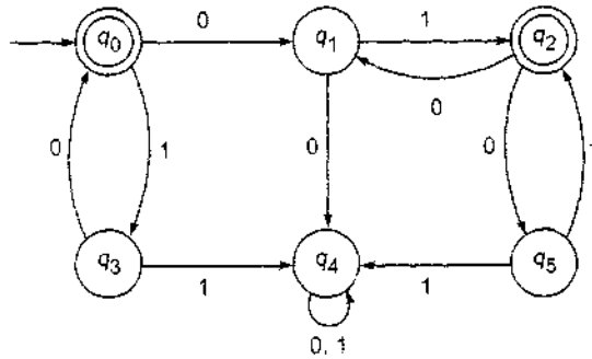
Fig. 3.22 DFA of Exercise 3.16.
