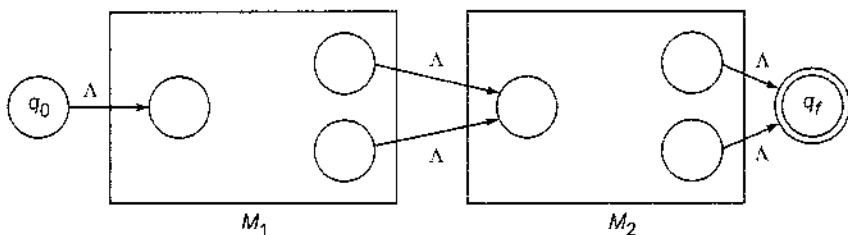
Fig. 5.8 NFA accepting L(PQ) .
