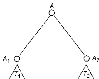
Fig. 6.12 Tree T with subtrees T_1 and T_2 .
