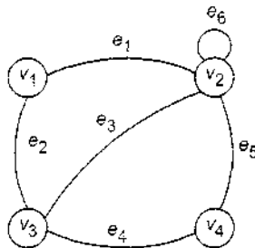
Fig. 2.3 An undirected graph.
