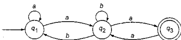
Fig. 5.13 Transition system of Example 5.8.
