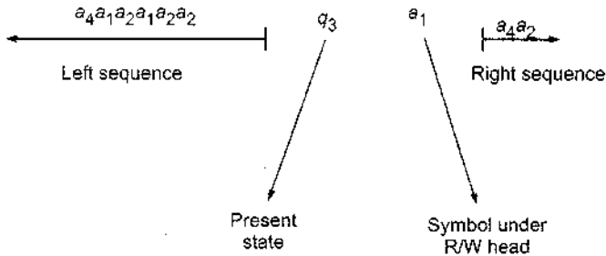
Fig. 9.3 Representation of ID.
