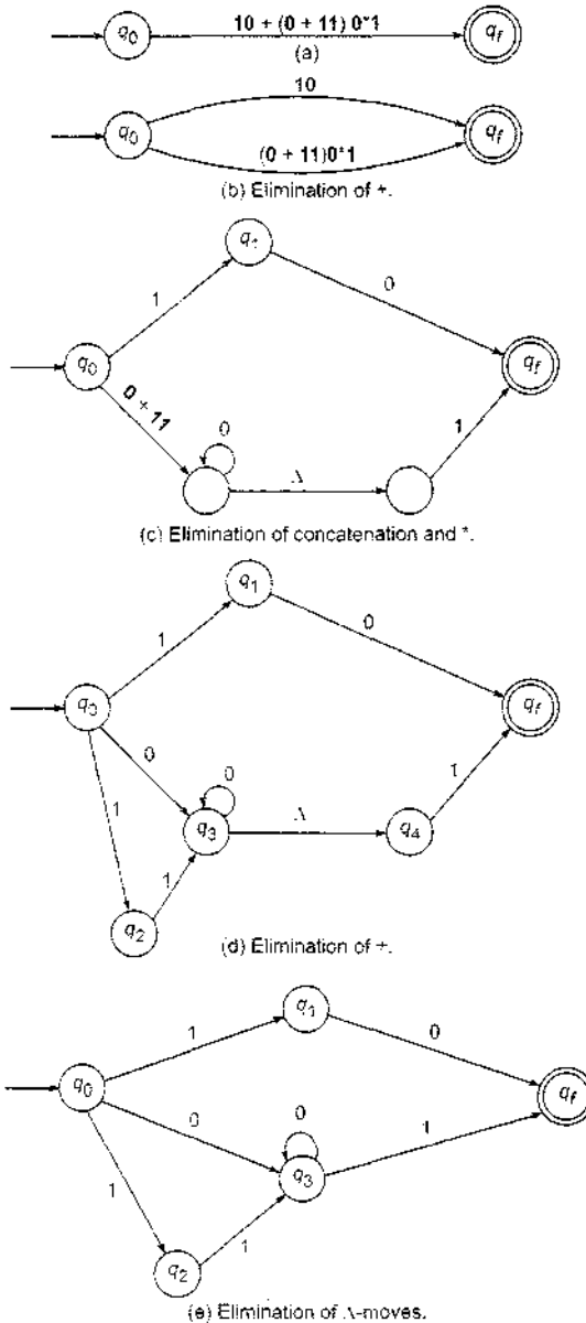
Fig. 5.21 Construction of finite automaton for Example 5.14.
