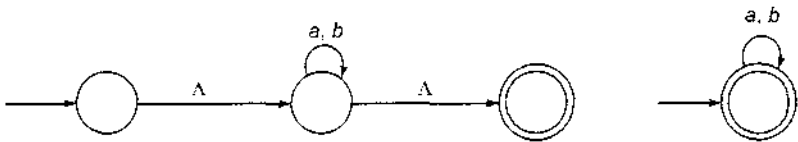
Fig. 5.25 Transition system for (a + b)^* .
