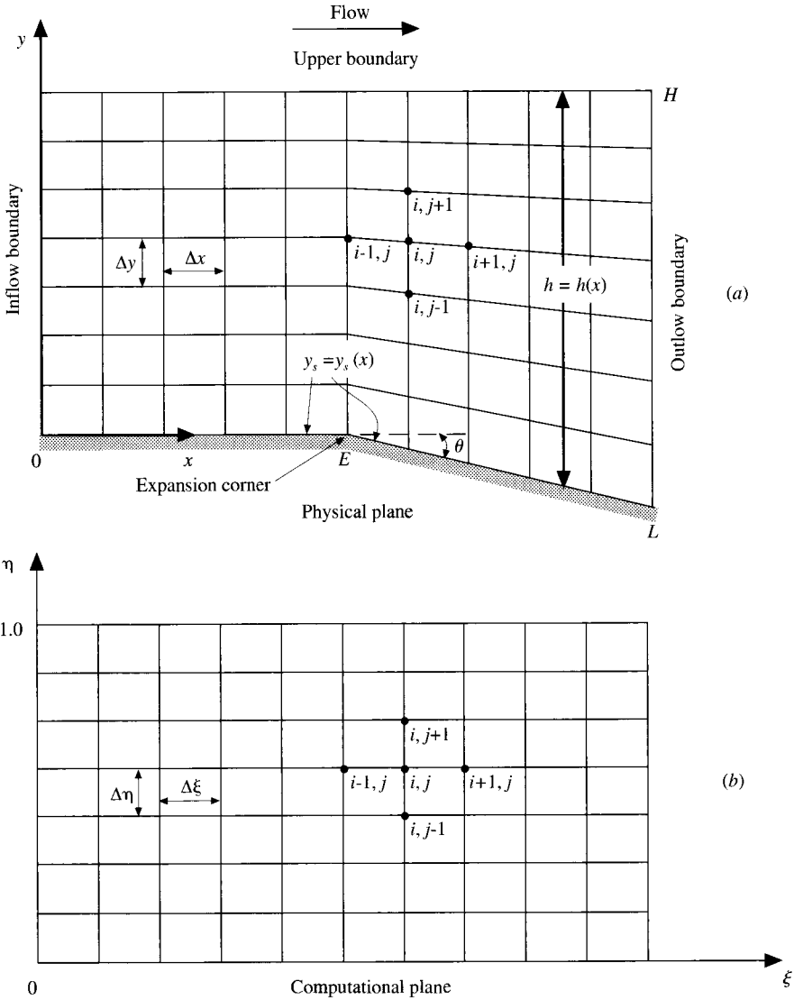
FIG. 8.3 The (a) physical and (b) computational planes for the numerical solution of the centered expansion wave problem.
