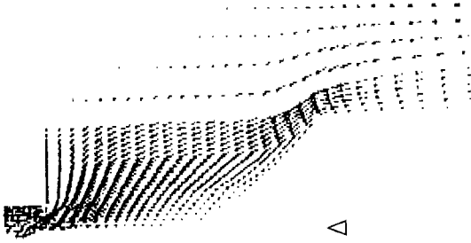
FIG. 1.19 Computed velocity field for the two-layer water and mud model shown in Fig. 1.18; results after 240 s of suction. (After Ref. 63.)
