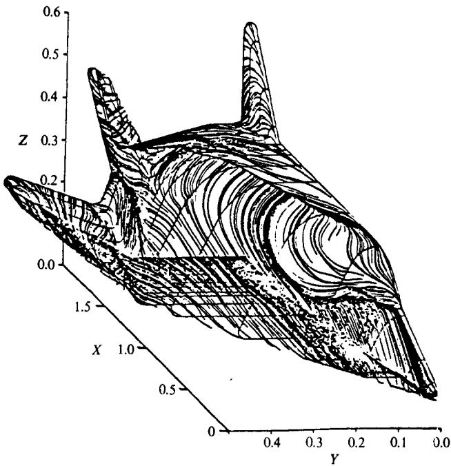
FIG. 12.2 Computed surface streamlines over the X-24C. (After Ref. 47.)
