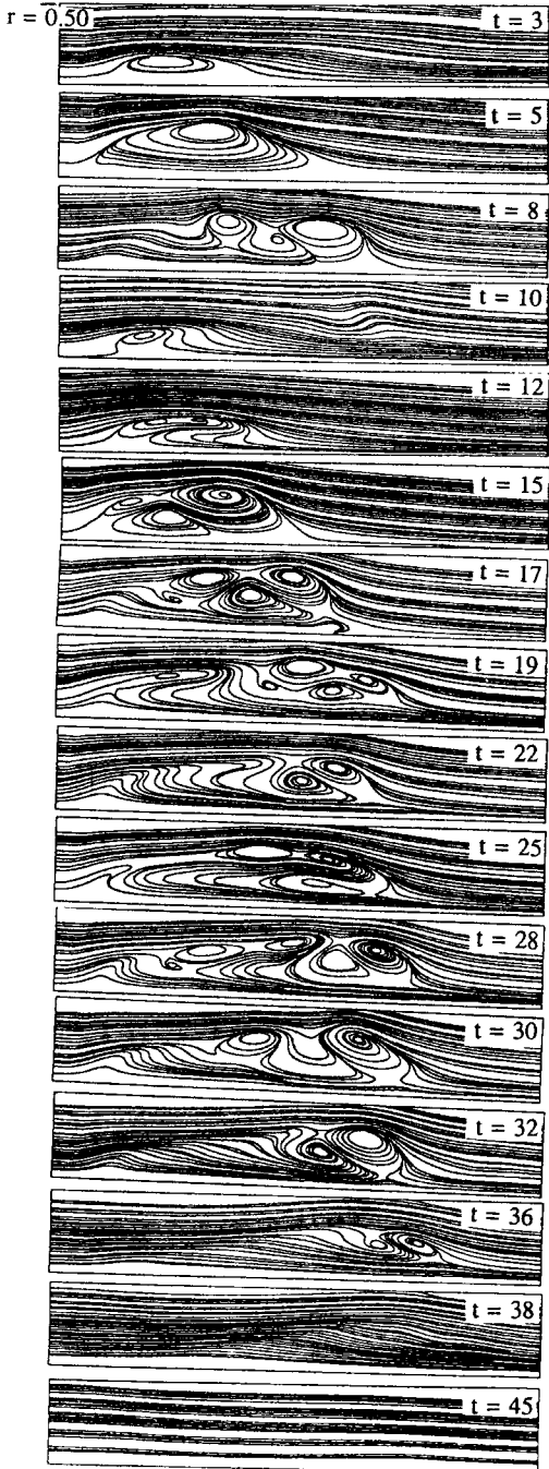
FIG. 12.12 Streamlines for a swirling flow that has passed through a shock wave (which is out of sight to the left). Flow is from left to right. Results show multibubble breakdown (vortex breakdown). (From Ref. 56. Copyright © 1991 AIAA. Reprinted with permission.)
