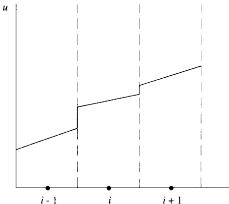
FIG. 11.10 Piecewise linear variation at time level n (second-order Godunov method.)
