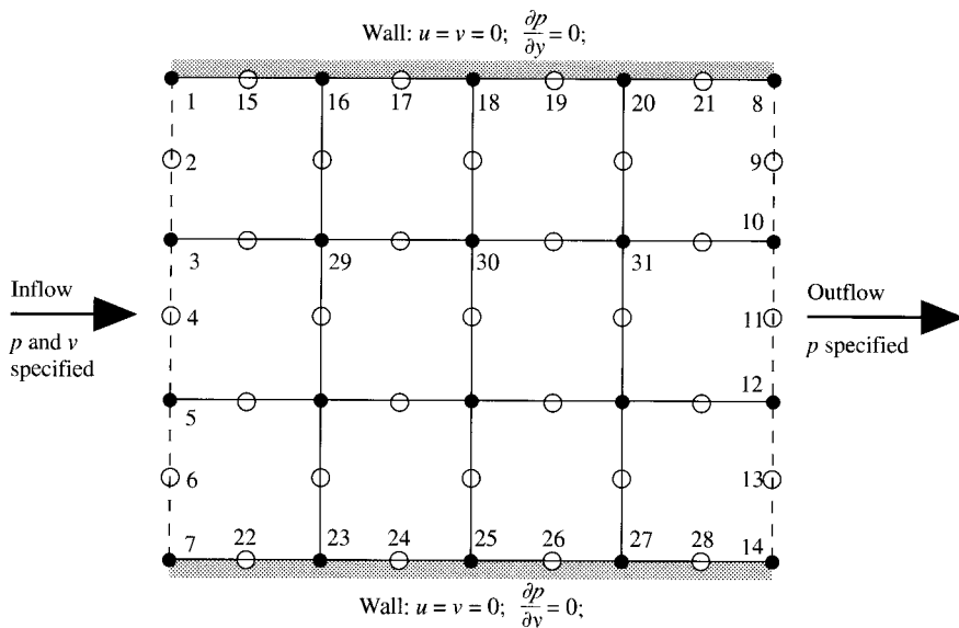
FIG. 6.18 Grid schematic for the discussion of boundary conditions for the pressure correction method.
