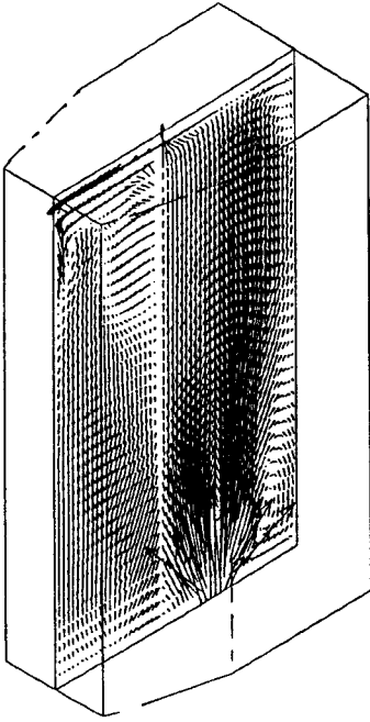
FIG. 1.21 Computed velocity field for the flow through the furnace in Fig. 1.20. Velocity vectors are shown emanating from points in a vertical perpendicular plane through the furnace. (From Ref. 64.)
