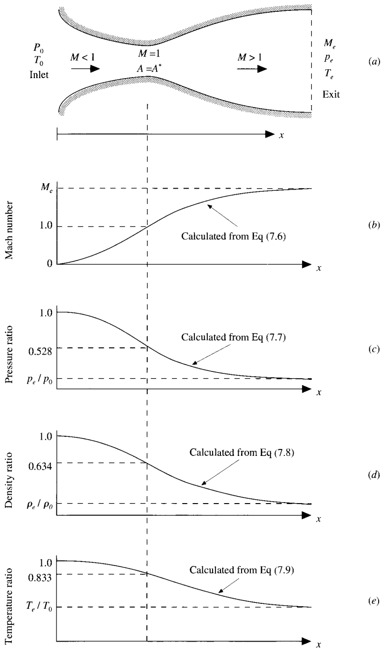
FIG. 7.2 Qualitative aspects of quasi-one-dimensional nozzle flow: isentropic subsonic-supersonic solution.
