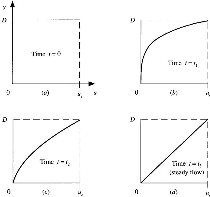
FIG. 9.2 Schematic of the velocity profiles at various times in an unsteady Couette flow.
