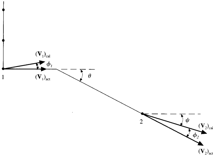
FIG. 8.5 Abbett's boundary condition for a steady flow.
