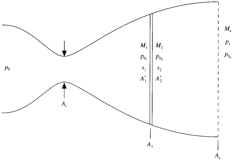
FIG. 7.22 Nomenclature for the normal shock case.
