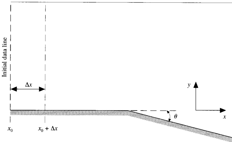
FIG. 8.2 Model for the downstream marching solution.
