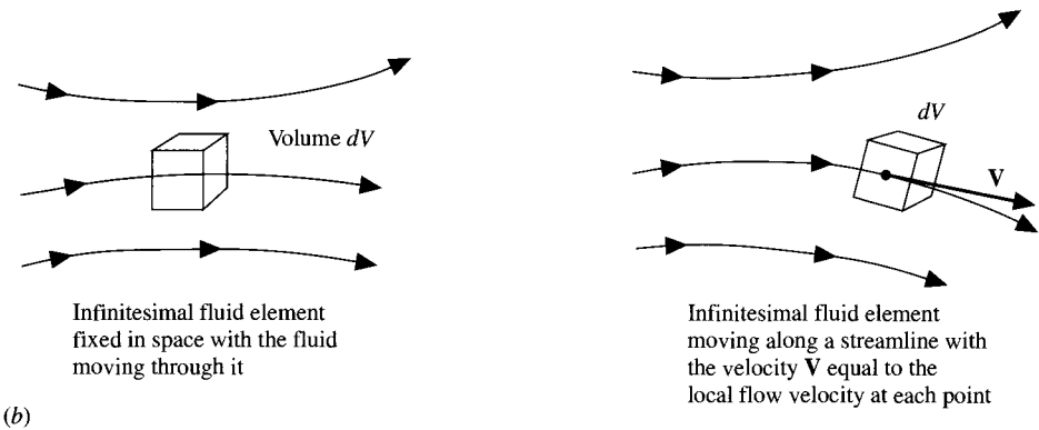
FIG. 2.2 Models of a flow. (a) Finite control volume approach; (b) infinitesimal fluid element approach.
