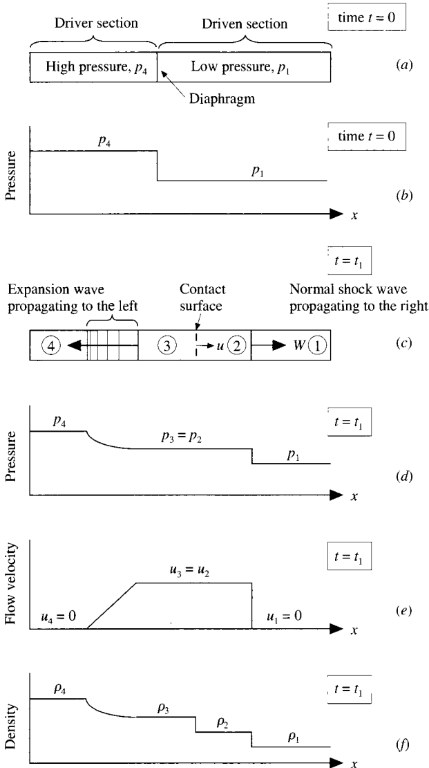
FIG. 11.5 Schematic of flow in a shock tube.
