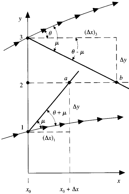
FIG. 8.6 Sketch in the physical plane for the calculation of the marching step size.
