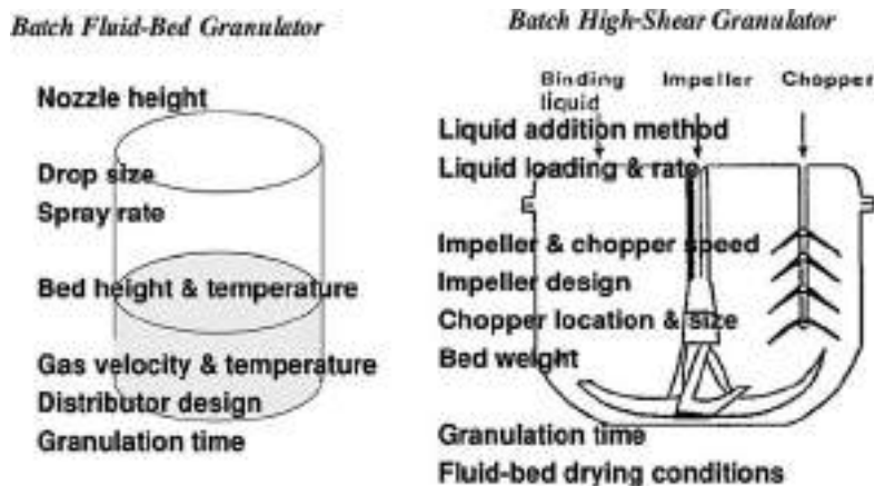
FIG. 21-87 Typical operating variable for granulation processes. (Reprinted from Design and Optimization of Granulation and Compaction Processes for Enhanced Product Performance, Ennis, 2006, with permission of E&G Associates. All rights reserved.)
