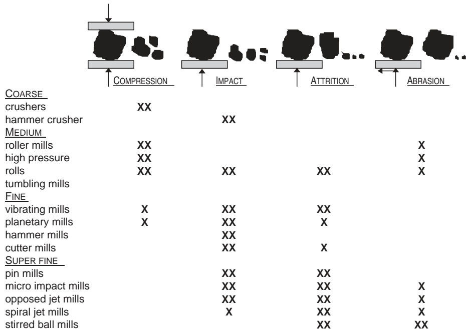
FIG. 21-60 Breakage modes in industrial mills. (Heiskanen, 1995.)
