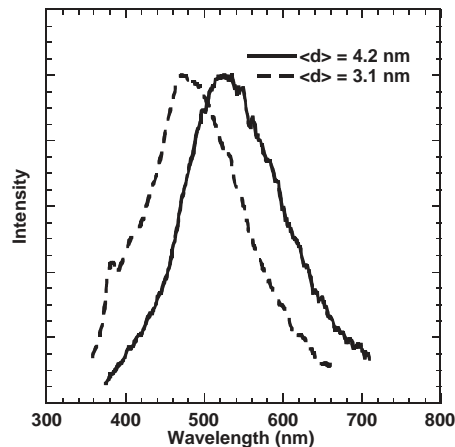
FIG. 20-23 Normalized photoluminescence spectra of 3.1-nm ( \lambda_{\text{excitation}} = 320 nm) and 4.2-nm ( \lambda_{\text{excitation}} = 340 nm) Ge nanoparticles dispersed in chloroform at 25°C with quantum yields of 6.6 and 4.6 percent, respectively. [Reprinted with permission from Lu et al., Nano Lett. , 4 (5), 969–974 (2004). Copyright 2004 American Chemical Society.]
