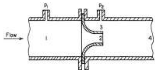
FIG. 10-19 Flow-nozzle assembly.
