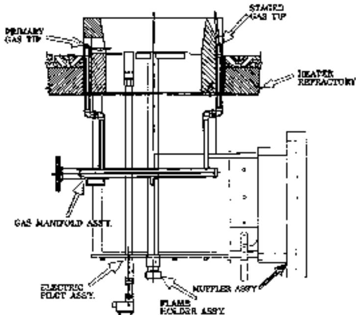
FIG. 24-33 Low-NO x fuel-staged burner for a natural draft refinery process heater. (Callidus Technologies, Inc.)
