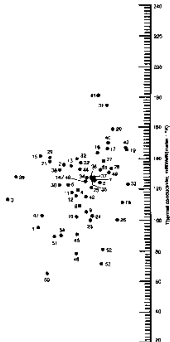
FIG. 2-33 and TABLE 2-320 Nomograph (right) for thermal conductivity of organic liquids. (From Mallu and Rao, Hydroc. Proc. 78, 1988.)
