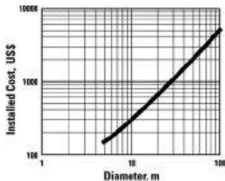
FIG. 18-106 Approximate installed cost of single-compartment thickeners (2005 US $).
