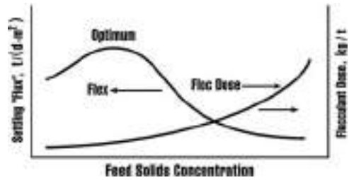
FIG. 18-99 Settling flux curve.
