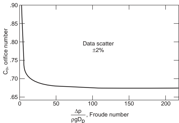
FIG. 6-19 Orifice coefficient vs. Froude number. (Courtesy E. I. duPont de Nemours &amp; Co.)
