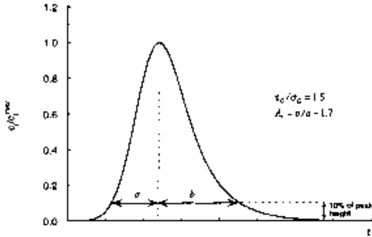
FIG. 16-32 Exponentially modified Gaussian peak with \tau_c/\sigma_c = 1.5 . The graph also shows the definition of the peak asymmetry factor A , at 10 percent of peak height.
