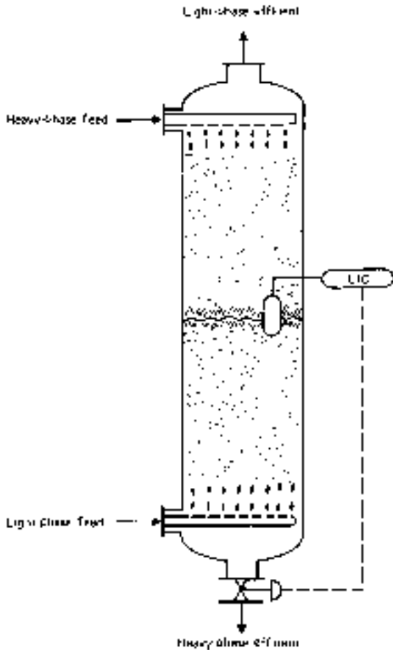
FIG. 15-34 Spray column with both phases dispersed.
