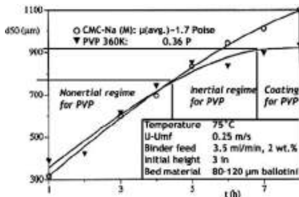
FIG. 21-120 Median granule diameter for fluid-bed granulation of ballotin with binders of different viscosity indicating regimes of growth [Ennis et al., Powder Technol. , 65 , 257 (1991)].
