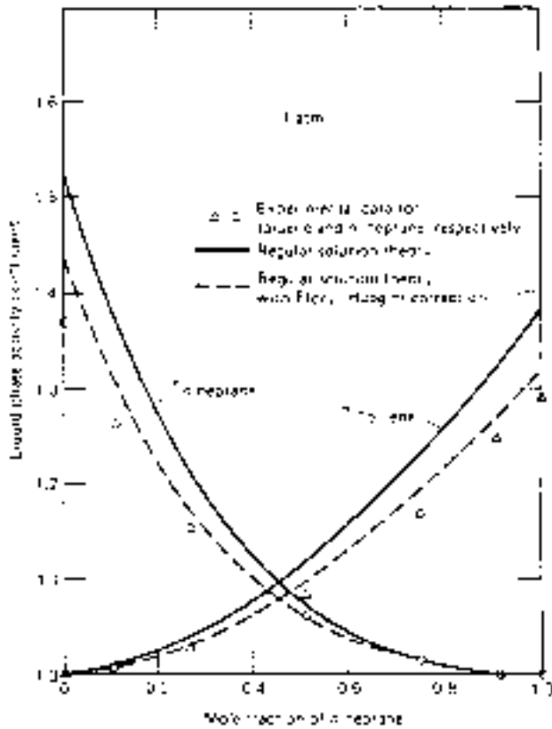
FIG. 13-14 Liquid-phase activity coefficients for an n -heptane-toluene system at 101.3 kPa (1 atm). [Henley and Seader, Equilibrium-Stage Separation Operations in Chemical Engineering , Wiley, New York, 1981; data of Yerezuniz et al., AIChE J. , 10 , 660 (1964).]
