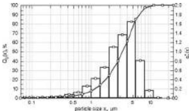
FIG. 21-2 Histogram \bar{q}_3(x) and Q_3(x) plotted with a logarithmic abscissa.
