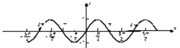
FIG. 3-39 Graph of y = \sin x .
