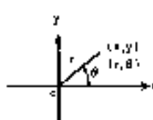
FIG. 3-13 Polar coordinates.
