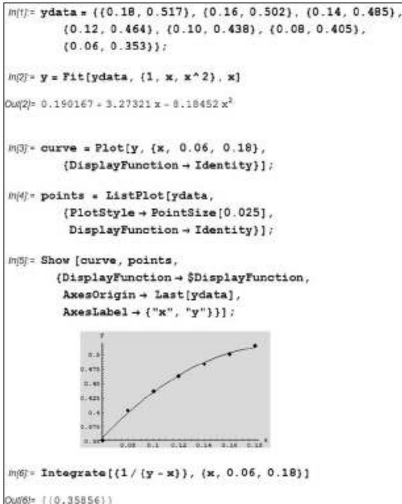
FIG. 13-118 Solution for a simple distillation example using Mathematica,® version 5.0.1.
