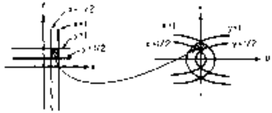
FIG. 3-47 Conformal transformation.
