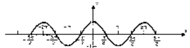
FIG. 3-40 Graph of y = \cos x .
