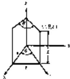
FIG. 3-26 Cylindrical coordinates.
