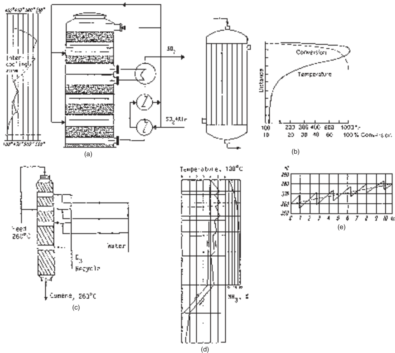
FIG. 19-22 Temperature and composition profiles. (a) Oxidation of \text{SO}_2 with intercooling and two cold shots. (b) Phosgene from \text{CO} and \text{Cl}_2 , activated carbon in 2-in tubes, water-cooled. (c) Cumene from benzene and propylene, phosphoric acid on quartz with four quench zones, 260^\circ\text{C} . (d) Vertical ammonia synthesizer at 300 atm, with five cold shots and an internal exchanger. (e) Vertical methanol synthesizer at 300 atm, \text{Cr}_2\text{O}_3\text{-ZnO} catalyst, with six cold shots totaling 10 to 20 percent of the fresh feed. To convert psi to kPa, multiply by 6.895; atm to kPa, multiply by 101.3.
