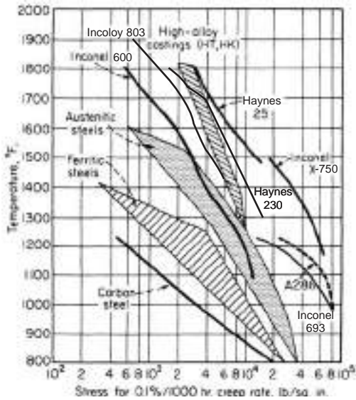
FIG. 25-21 Effect of creep on metals for high-temperature use. °C = (°F - 32) × 5/9; to convert lbf/in 2 to MPa, multiply by 6.895 × 10 -3 . [Chem. Eng., 65, p. 140 (Dec. 15, 1958); modified 2005 using producer data.]
