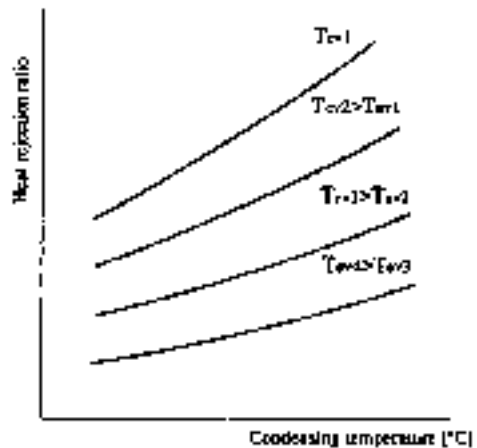
FIG. 11-94 Heat-rejection ratio.
