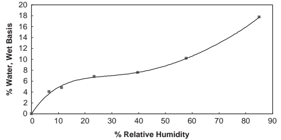
FIG. 12-11 Example of a sorption isotherm (coffee at 22°C).
