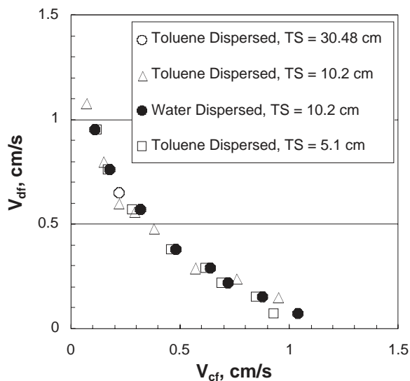
FIG. 15-43 Effect of tray spacing on baffle tray capacity. [Taken from Seibert, Lewis, and Fair, Paper No. 112a, AIChE National Meeting , Indianapolis (November 2002), with permission. Copyright 2002 AIChE.]
