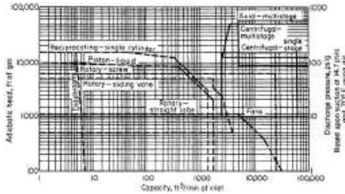
FIG. 10-64 Compressor coverage chart based on the normal range of operation of commercially available types shown. Solid lines: use left ordinate, head. Broken lines: use right ordinate, pressure. To convert cubic feet per minute to cubic meters per hour, multiply by 1.699; to convert feet to meters, multiply by 0.3048; and to convert pounds-force per square inch to kilopascals, multiply by 6.895; (^{\circ}\text{F} - 32)/1.8 = ^{\circ}\text{C} .
