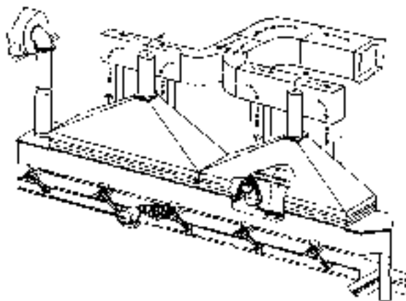
FIG. 12-65 Vibrating conveyor dryer. (Carrier Vibrating Equipment, Inc.)
