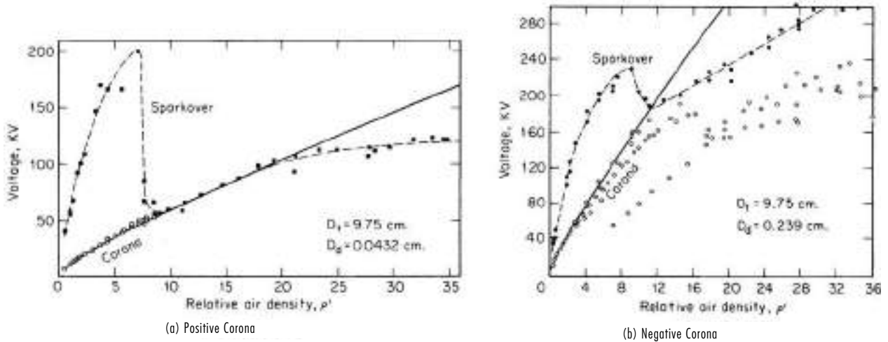
FIG. 17-67 Corona-starting and sparkover voltages for coaxial wire-pipe electrodes in air (25°C). D_1 and D_2 are the respective pipe and wire diameters. The voltage is unvarying direct current. (Robinson, Air Pollution Control, part 1 , Wiley-Interscience, New York, 1971, chap. 5.)
