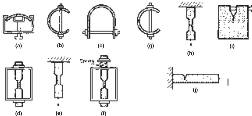
FIG. 25-17 Specimens for stress-corrosion tests. (a) Bent beam. (b) C ring. (c) U bend. (d) Tensile. (e) Tensile. (f) Tensile. (g) Notched C ring. (h) Notched tensile. (i) Precracked, wedge open-loading type. (j) Precracked, cantilever beam. [Chem. Eng., 78, 159 (Sept. 20, 1971).]
