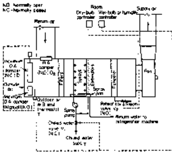
FIG. 11-69 Typical central-station air-conditioning unit and control system. On a rising room wet-bulb temperature, the wet-bulb branch-line air pressure increases through the reverse-acting outdoor-air wet-bulb temperature-limit thermostat T_1 to open gradually the maximum outdoor-air damper D_1 and simultaneously close return-air damper D_2 , then gradually open chilled-water valve V_1 . On a rising room dry-bulb temperature, the dry-bulb branch-line air pressure gradually increases to close reheat steam valve V_2 . When outdoor wet-bulb temperature exceeds the set point of the outdoor-air wet-bulb-limit thermostat T_1 , which is set at the return-air wet-bulb temperature, this thermostat decreases branch-line pressure to close gradually maximum outdoor damper D_1 and simultaneously open return-air damper D_2 . The reverse sequences are followed during the heating season.
