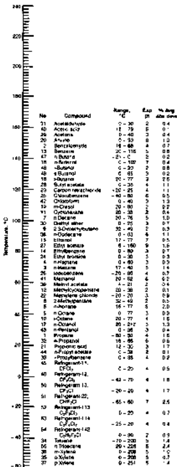
FIG. 2-33 and TABLE 2-320 Nomograph (right) for thermal conductivity of organic liquids. (From Mallu and Rao, Hydroc. Proc. 78, 1988.)
