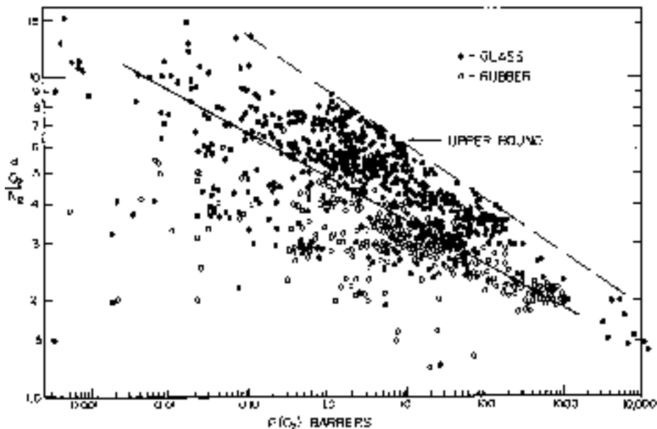
FIG. 20-69 Plot of separation factor versus permeability for many polymers, O 2 /N 2 . Abscissa—"Fast Gas Permeability, \rho (O 2 ) Barrers." Ordinate—"Selectivity, \alpha (O 2 /N 2 )."
