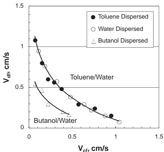
FIG. 15-42 Capacity characteristics of a baffle tray extractor. Tray overlap = 62 percent. Column diameter = 10.2 cm. [Taken from Seibert, Lewis, and Fair, Paper No. 112a, AIChE National Meeting , Indianapolis (November 2002), with permission. Copyright 2002 AIChE.]
