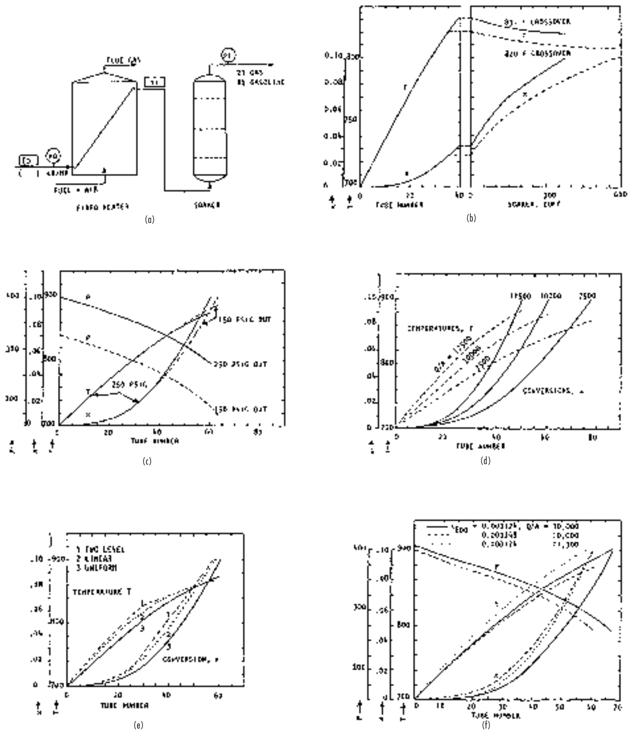
FIG. 19-12 (a) Visbreaking flow sketch, feed 160,000 lbm/h, k_{500} = 0.000248/s , tubes 5.05-in ID by 40 ft. (b) Q/A = 10,000 Btu/(ft 2 -h), P_{out} = 250 psig. (c) Q/A = 10,000 Btu/(ft 2 -h), P_{out} = 150 or 250 psig. (d) Three different heat fluxes, P_{out} = 250 psig. (e) Variation of heat flux, average 10,000 Btu/(ft 2 -h), P_{out} = 250 psig. (f) Halving the specific rate. T in °F. To convert psi to kPa, multiply by 6.895; ft to m, multiply by 0.3048; in to cm, multiply by 2.54.
