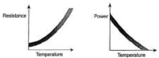
FIG. 10-185 Self-regulation.
