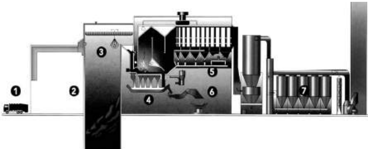
FIG. 22-53 1200-tons/day MSW plant schematic.
