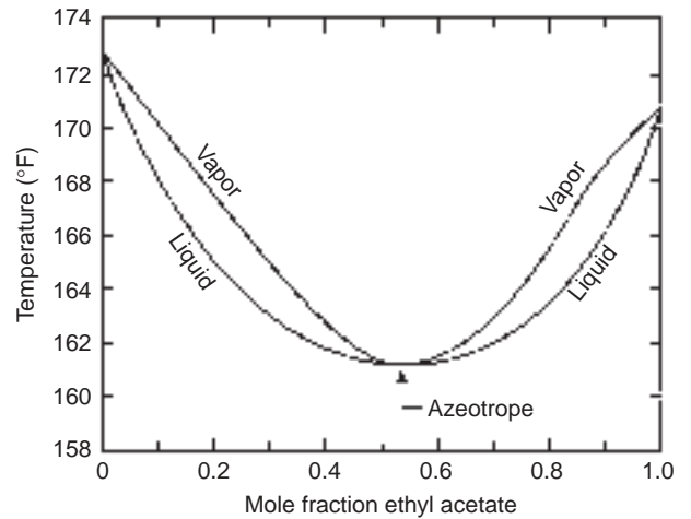
FIG. 13-6 Liquid boiling points and vapor condensation temperatures for minimum-boiling azeotrope mixtures of ethyl acetate and ethanol at 101.3-kPa (1-atm) total pressure.
