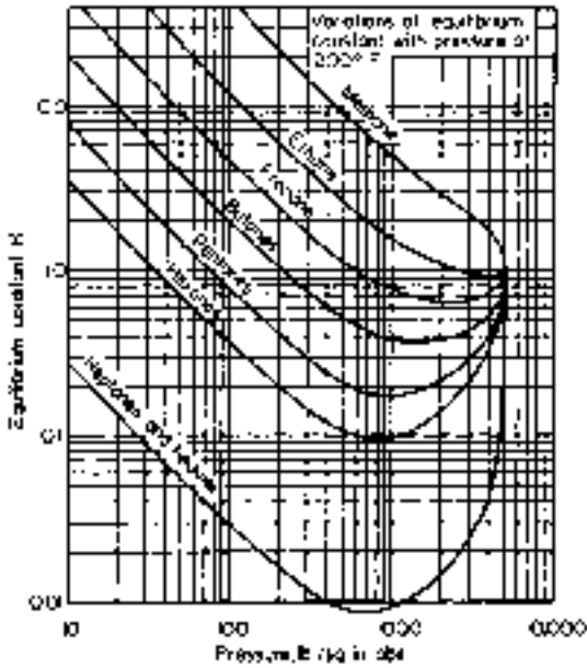
FIG. 13-10 Typical variation of K values with total pressure at constant temperature for a complex mixture. Light hydrocarbons in admixture with crude oil. [Katz and Hachmuth, Ind. Eng. Chem. , 29 , 1072 (1937).]
