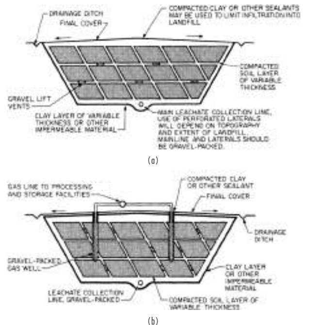
FIG. 22-63 Use of an impermeable liner to control the movement of gases and leachate in landfills. (a) Without gas recovery. (b) With gas recovery. (From C. Tchobanoglous, H. Theisen, and R. Eliassen, Solid Wastes: Engineering Principles and Management Issues , McGraw-Hill, New York, 1977.)
