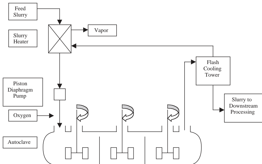
FIG. 18-90 Three-compartment autoclave.
