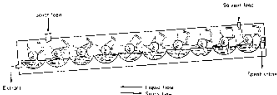
FIG. 18-87 Kennedy extractor. (Vulcan Cincinnati, Inc.)
