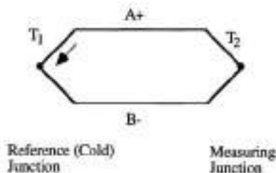
FIG. 8-63 Basic circuit of Seebeck effect.
