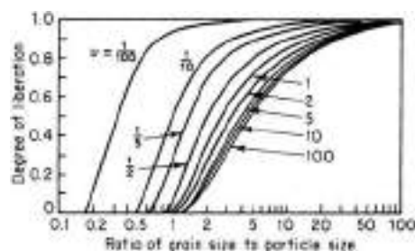
FIG. 21-63 Fraction of mineral B that is liberated as a function of volumetric abundance ratio v of gangue to mineral B ( 1/\text{grade} ), and ratio of grain size to particle size of broken fragments ( 1/\text{fineness} ). [Wiegel and Li, Trans. Soc. Min. Eng.-Am. Inst. Min. Metall. Pet. Eng. , 238 , 179 (1967).]
