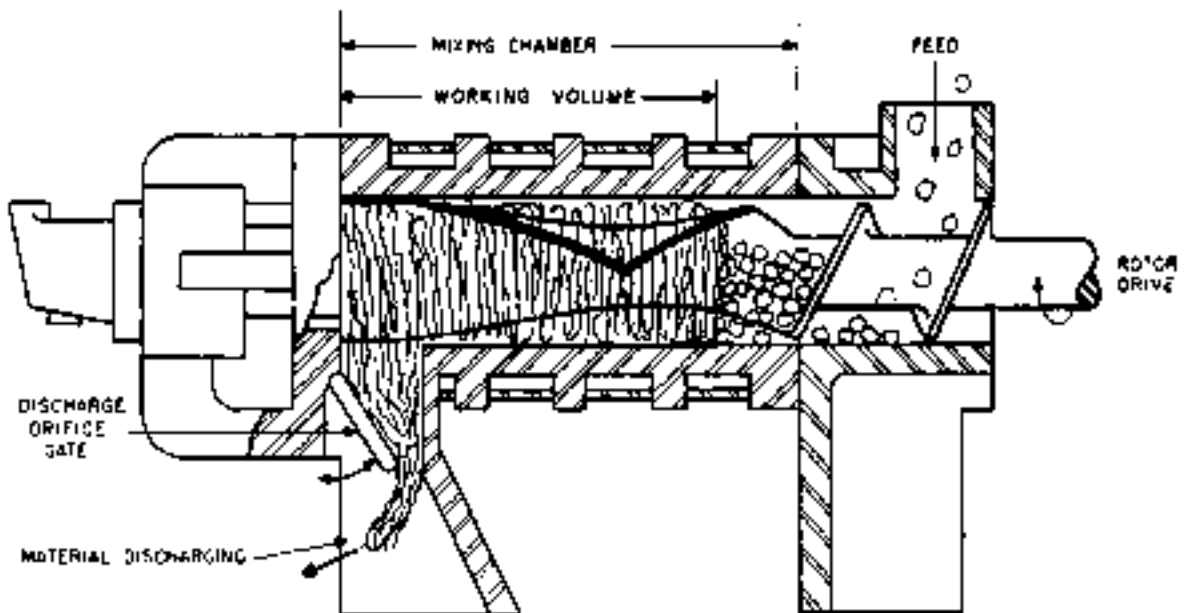
FIG. 18-58 Farrel continuous mixer. (Farrel Co.)
