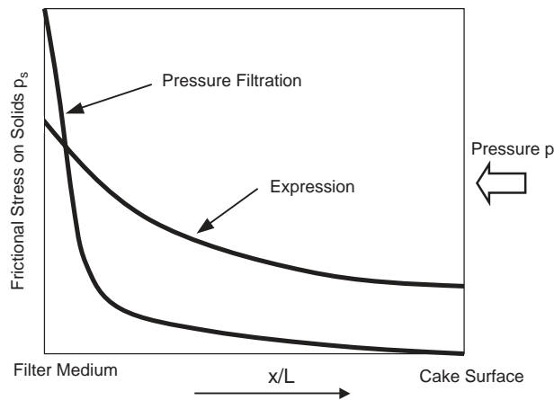
FIG. 18-185 Comparisons of frictional stress distributions in expression and pressure filtration.
