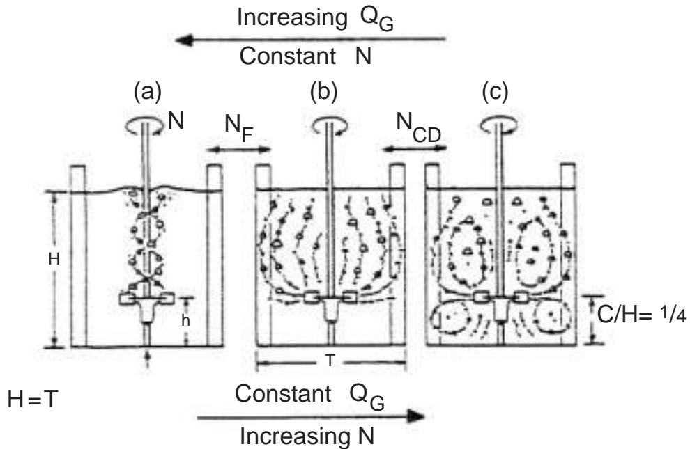
FIG. 19-34 Gas circulation as a function of stirrer speed. (From Nienow et al., 5th European Conference on Mixing, Wurzburg, 1985; published by BHRA, The Fluid Engineering Centre, Cranfield, England; Fig. 1.)
