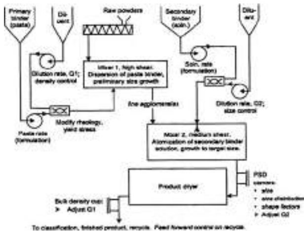
FIG. 21-165 Two-stage continuous granulation process, consisting of high-shear nucleation (pin mixer) and moderate shear growth and consolidation (plough shear). [Mort et al., Powder Technol., 117, 173 (2003).]
