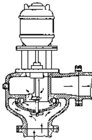
FIG. 18-35 Nettco Corp. Flomix.
