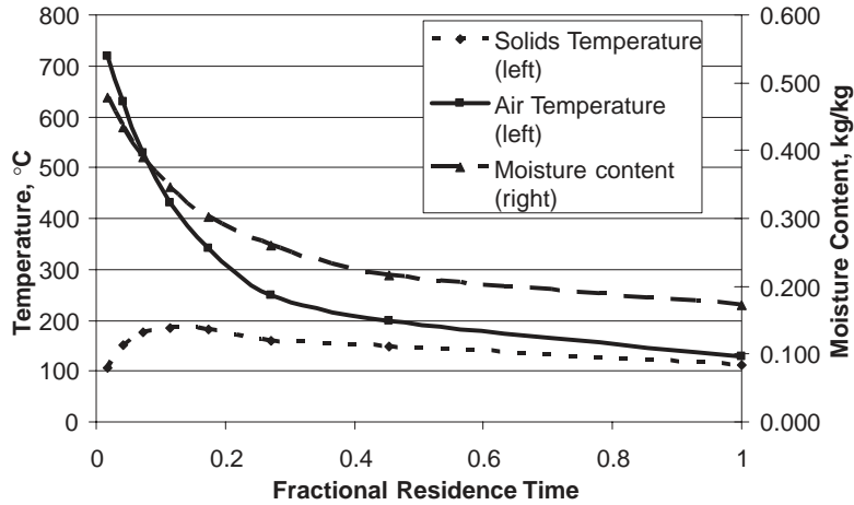
FIG. 12-42 Typical variation of process conditions through a cocurrent cascading rotary dryer.
