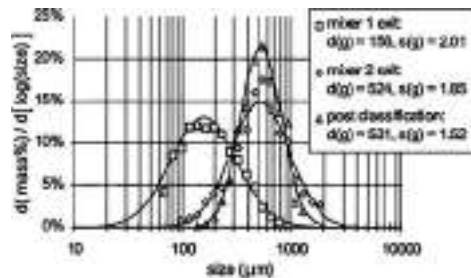
FIG. 21-166 Two-stage continuous granulation process, consisting of high-shear nucleation (pin mixer) and moderate shear growth and consolidation (plough shear). Exit granule size distributions are determined by in-line imaging. [Mort et al., Powder Technol., 117, 173 (2003).]
