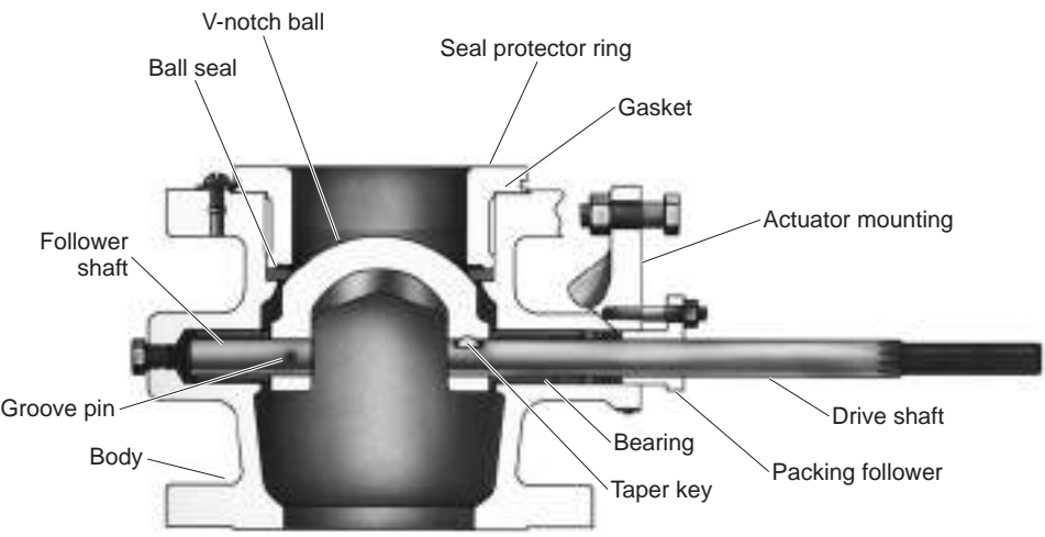
FIG. 8-69 Segmented ball valve. Partial view of actuator mounting shown 90° out of position. (Courtesy Fisher Controls International LLC.)
