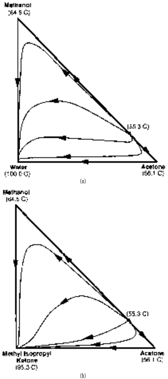
FIG. 13-93 Residue curve maps for acetone-methanol systems. (a) With water. (b) With MIPK.
