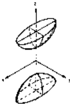
FIG. 3-31 Hyperboloid of two sheets. \frac{x^2}{a^2} + \frac{y^2}{b^2} - \frac{z^2}{c^2} = -1
