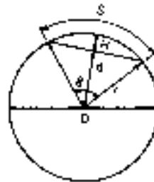
FIG. 3-5 Circle.
