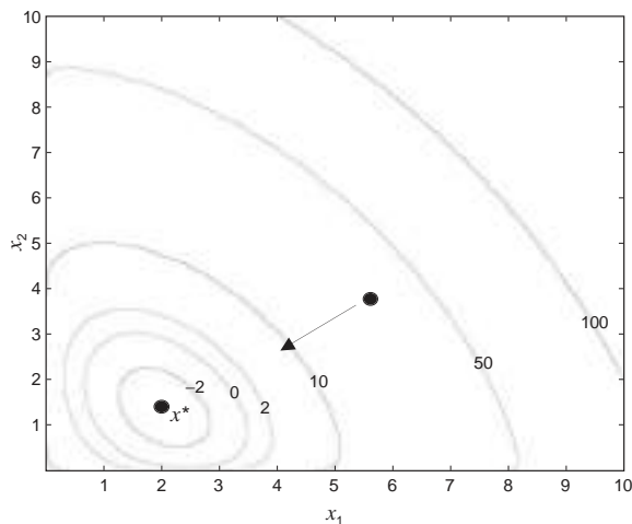
FIG. 3-54 Unconstrained minimum.
