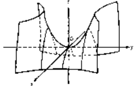
FIG. 3-34 Hyperbolic paraboloid. \frac{x^2}{a^2} - \frac{y^2}{b^2} + cz = 0
