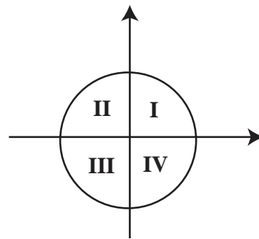
FIG. 3-37 Quadrants.
