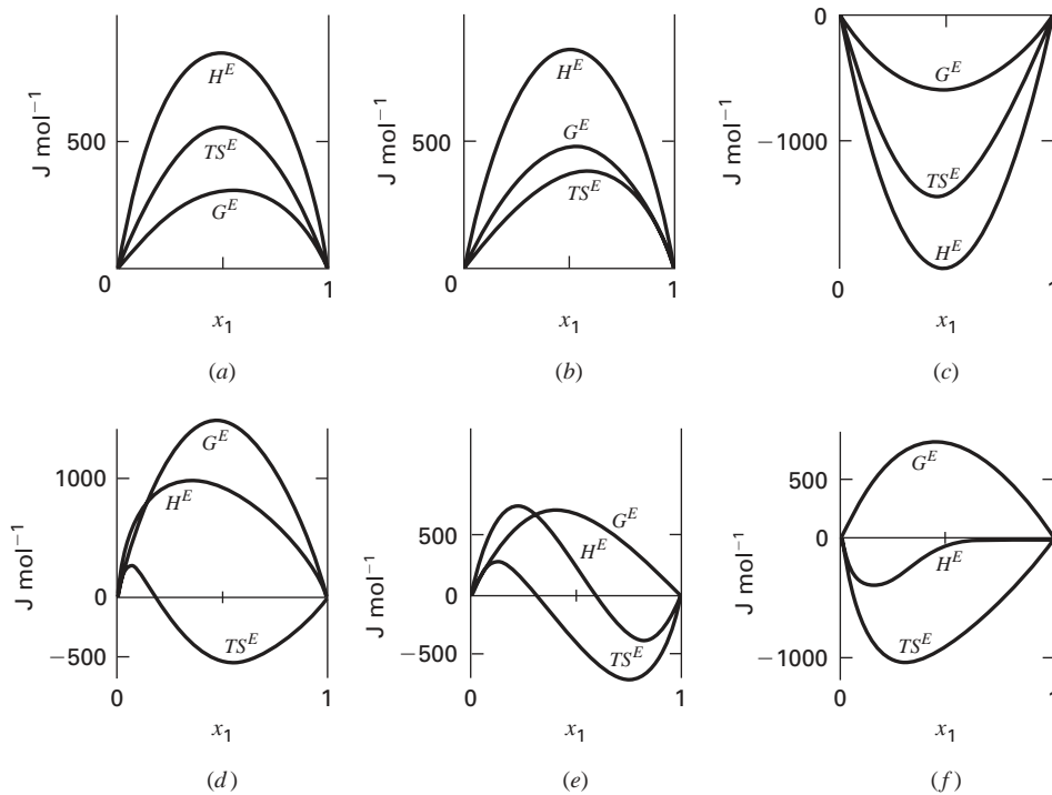
FIG. 4-5 Excess properties at 50°C for six binary liquid systems: (a) chloroform(1)/ n -heptane(2); (b) acetone(1)/methanol(2); (c) acetone(1)/chloroform(2); (d) ethanol(1)/ n -heptane(2); (e) ethanol(1)/chloroform(2); (f) ethanol(1)/water(2). [Smith, Van Ness, and Abbott, Introduction to Chemical Engineering Thermodynamics , 7th ed., p. 420, McGraw-Hill, New York (2005).]
