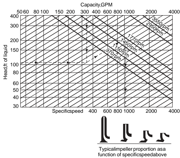
FIG. 10-46 Relationships between specific speed, rotative speed, and impeller proportions ( Worthington Pump Inc., Pump World, vol. 4, no. 2, 1978 ).
