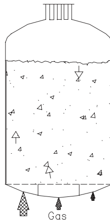
fluid bed mixer
