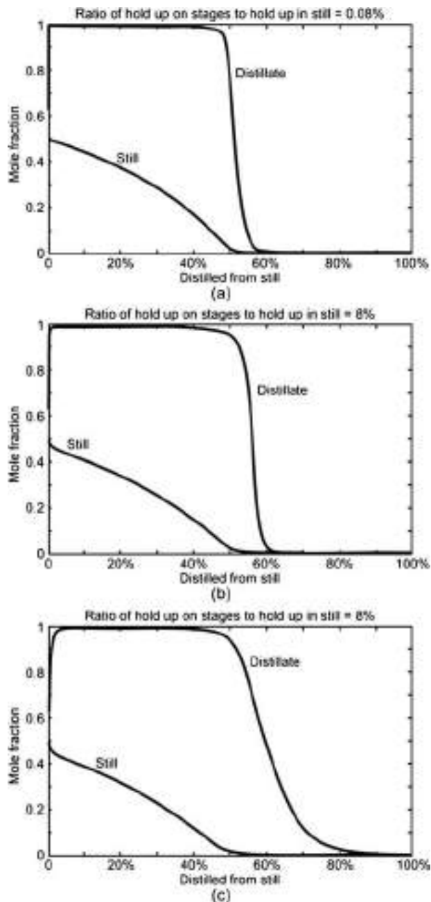
FIG. 13-127 Effects of holdup on batch rectifier.
