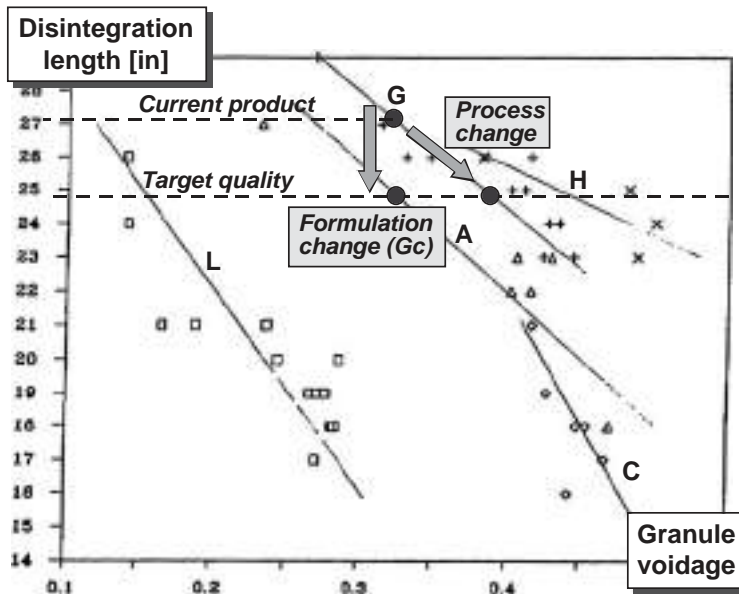
FIG. 21-90 Impact of granule voidage on dissolution. (After Maroglou, reprinted from Design and Optimization of Granulation and Compaction Processes for Enhanced Product Performance, Emis , 2006, with permission of E&G Associates. All rights reserved.)
