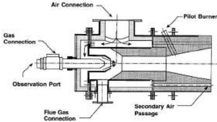
FIG. 24-32 Low-NO x burner with air-staging and flue-gas recirculation for use in high-temperature furnaces. (Hauck Manufacturing Company. Developed and patented by the Gas Research Institute.)
