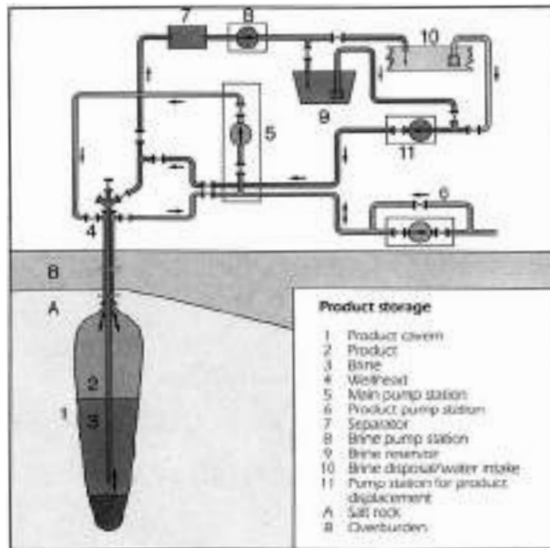
FIG. 10-191 Brine-compensated storage.
