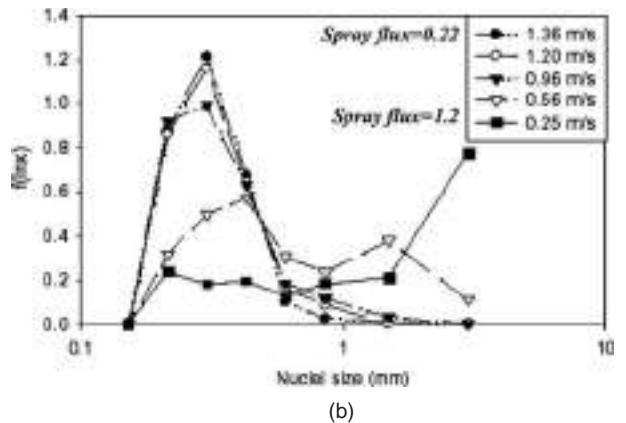
FIG. 21-105 Effect of (a) spray drop distribution (b) low spray flux—water and HPC and (b) powder velocity (variable spray flux—water) on nuclei size distribution. Lactose feed powder in spinning granulator. (Litster and Emnis, loc. cit.)
