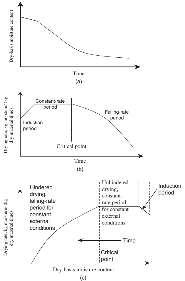
FIG. 12-13 Several common representations of a typical drying curve.
