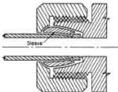
FIG. 10-148 Bite-type-fitting joint.
