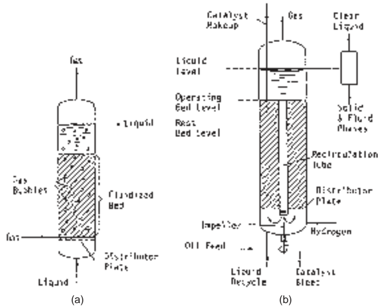
FIG. 19-39 Gas-liquid-solid reactors. (a) Three-phase fluidized-bed reactor for hydroliquefaction of coal. (Kampiner, in Winnacker-Keuchler, Chemische Technologie , vol. 3, Hanser, 1972, p. 252.)
