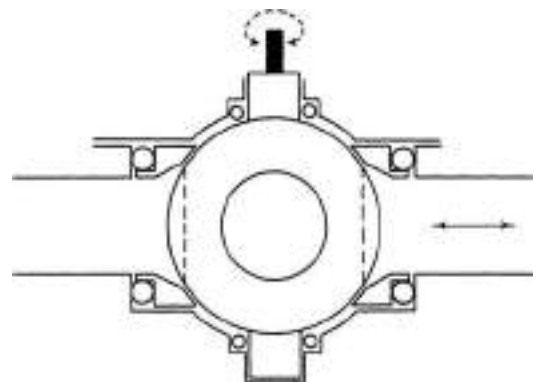
FIG. 10-157 Ball valve; trunnion-mounted ball.
