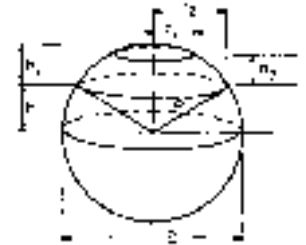
FIG. 3-10 Sphere.
