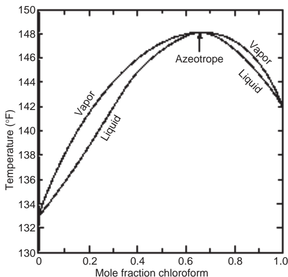
FIG. 13-7 Liquid boiling points and vapor condensation temperatures for maximum-boiling azeotropic mixtures of chloroform and acetone at 101.3-kPa (1-atm) total pressure.
