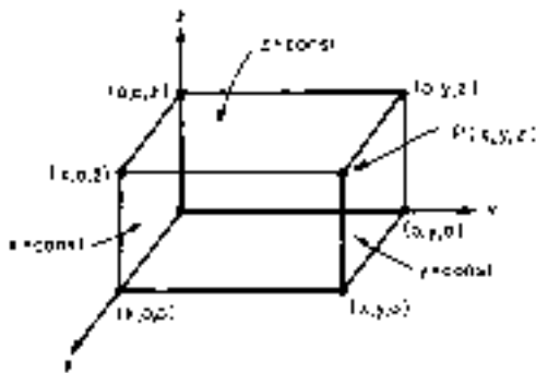
FIG. 3-25 Cartesian coordinates.
