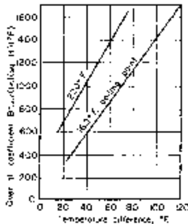
FIG. 11-24 Heat-transfer coefficients for seawater in coil-tube evaporators. ^{\circ}\text{C} = (^{\circ}\text{F} - 32)/1.8 ; to convert British thermal units per hour-square foot-degrees Fahrenheit to joules per square meter-second-kelvins, multiply by 5.6783.
