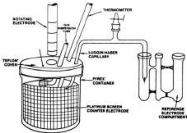
FIG. 25-15 Rotating cylinder electrode apparatus.
