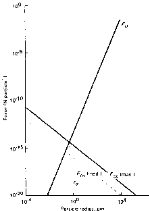
FIG. 20-31 Comparison of the dielectrophoretic ( F_{\text{DEP}} ) and osmotic ( F_{\text{os}} ) forces as functions of the particle size.
