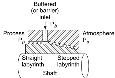
(f) Buffered combination labyrinth
