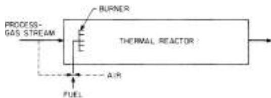
FIG. 22-13 Thermal-combustion device.
