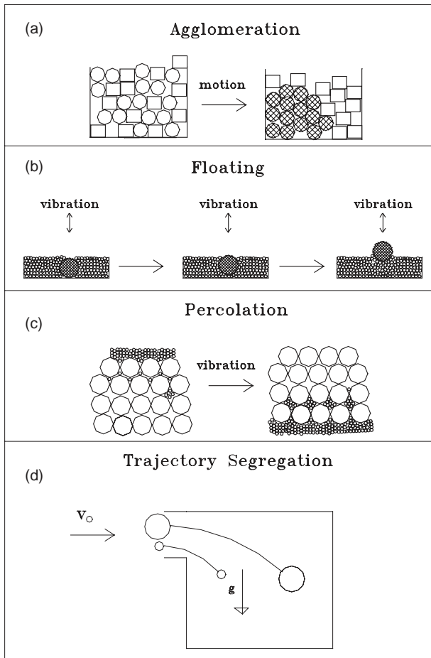
FIG. 21-43 Four mechanisms of segregation, following Williams.
