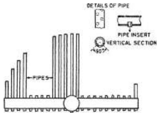
FIG. 17-12 Multiple-pipe gas distributor. [From Sternerding, de Groot, and Kuypers, Soc. Chem. Ind. J. Symp. Fluidization Proc., 35-46, London (1963).]
