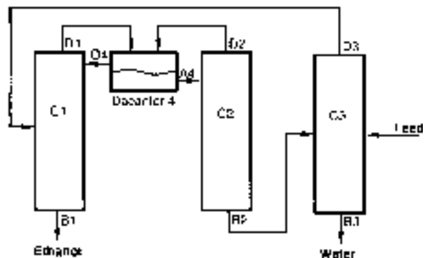
FIG. 13-90 Three-column sequence for ethanol dehydration with cyclohexane (operating column C2 in the direct-split mode).
