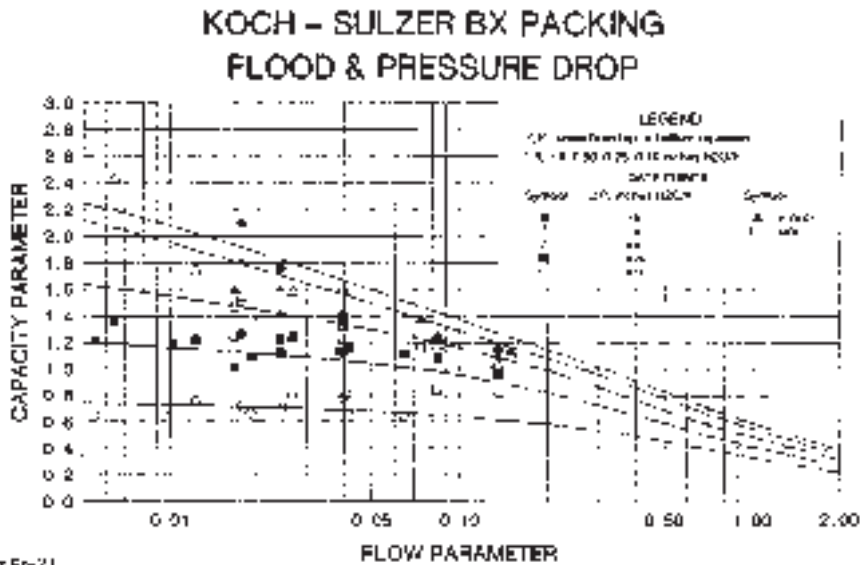
Basic Fp-21 Pressure drop measured in inches H 2 O/ft Large symbols represent non-bubbly data
