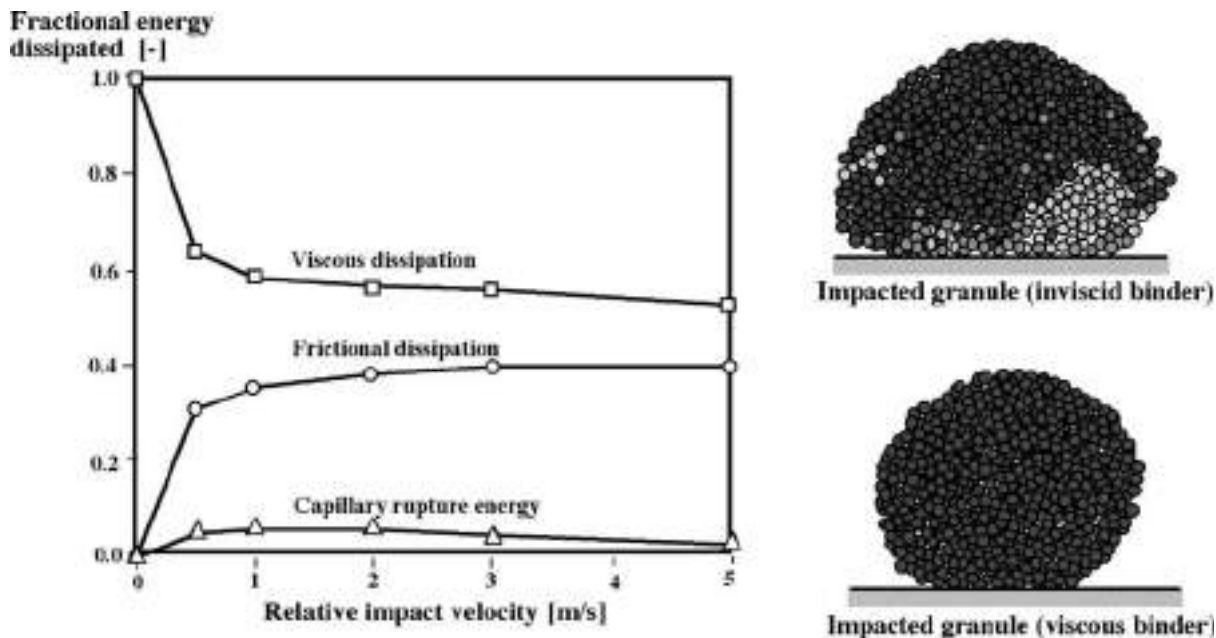
FIG. 21-116 Distribution of energy dissipation during agglomerate collisions, with granular simulations of wall impact for 128- \mu s duration for inviscid and viscous binder agglomerates. [After Adams, Thornton, and Lian, Agglomeration and Size Enlargement , Proc. 1st Int. Particle Technology Forum, vol.1, Denver, Colo., AIChE, New York, 1994, pp. 155–286, with permission.]
