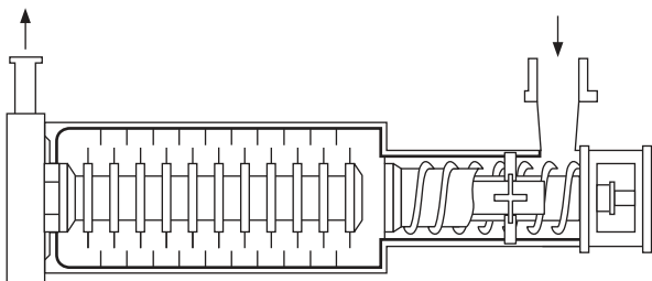
FIG. 21-75 Drais wet-grinding and dispersing system (U.S. patent 3,957,210) Draiserwerke GmbH. [ Stein , International J. Mineral Processing, 22 (1-4), 431-444 (1988).]
