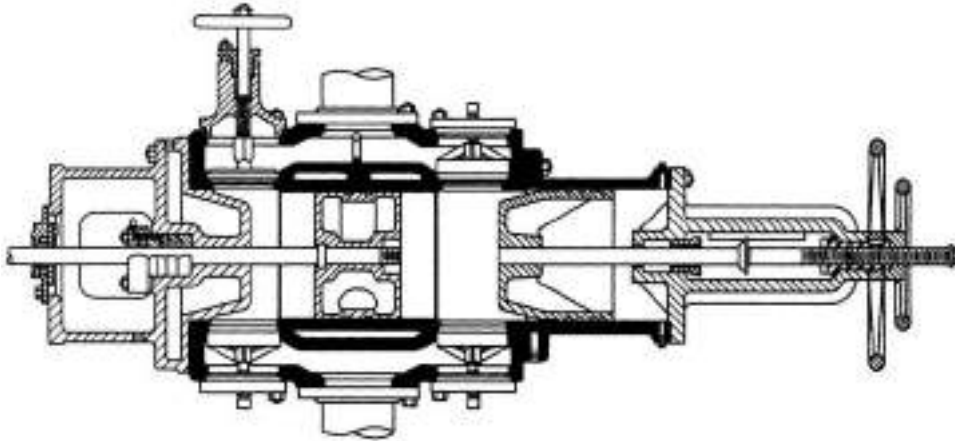
FIG. 10-75 Sectional view of a cylinder equipped with a hand-operated valve lifter on one end and a variable-volume clearance pocket at other end.
