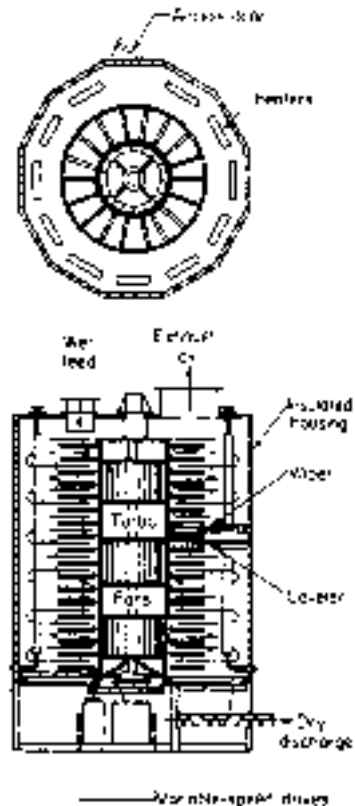
FIG. 12-45 TURBO-DRYER®. (Wyssmont Company, Inc.)
