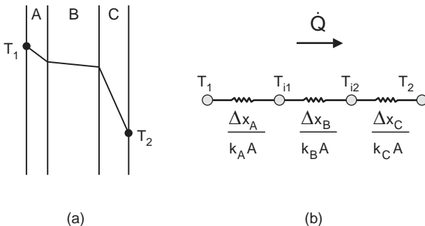
FIG. 5-3 Steady-state temperature profile in a composite wall with constant thermal conductivities k_A , k_B , and k_C and no energy sources in the wall. The thermal circuit is shown in (b). The total resistance is the sum of the three resistances shown.
