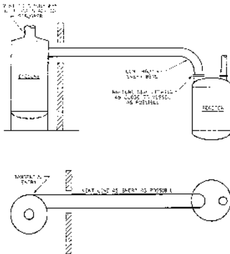
FIG. 23-54 Cyclone separator with integral catch tank.
