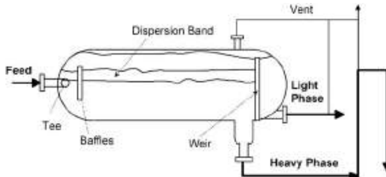
FIG. 15-64 Typical horizontal gravity decanter design.
