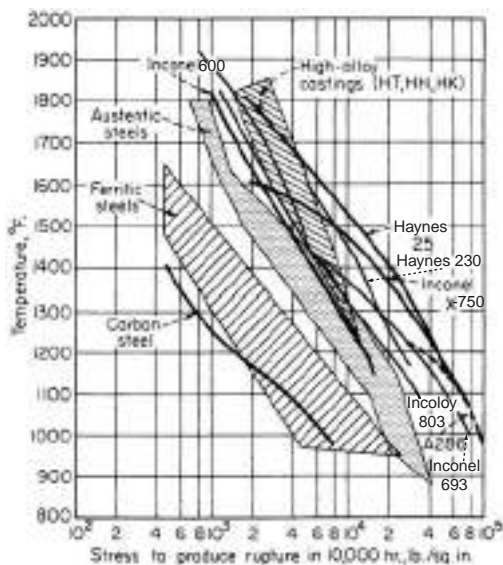
FIG. 25-22 Rupture properties of metals as a function of temperature. °C = (°F - 32) × 5/9; to convert lbf/in 2 to MPa, multiply by 6.895 × 10 -3 . [Chem. Eng., 65, p. 140 (Dec. 15, 1958); modified 2005 using producer data.]
