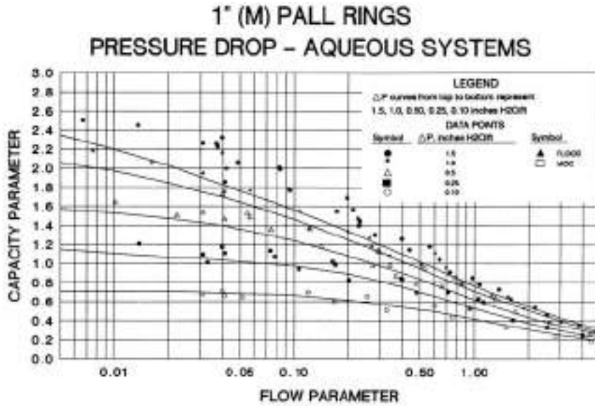
Basic Fp-56 Pressure drop measured in inches H 2 O/ft
