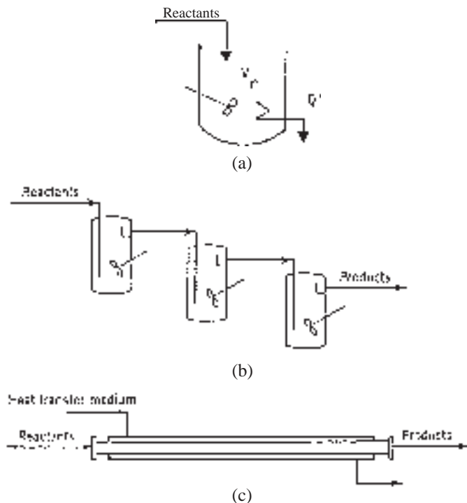
FIG. 7-1 Types of ideal reactors: (a) Batch or semibatch. (b) CSTR or series of CSTRs. (c) Plug flow.
