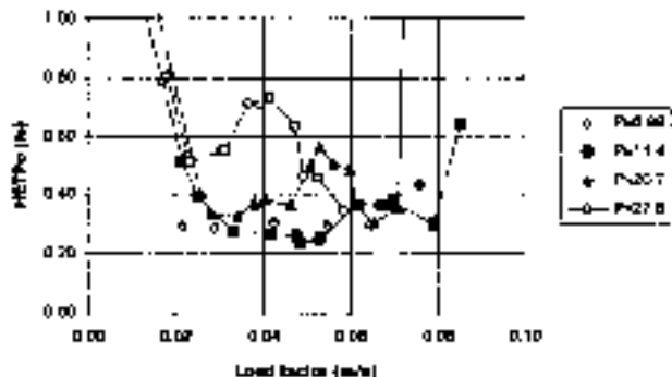
FIG. 14-62 HETP o data as measured in the FRI column for the i C 4 / n C 4 system at different pressures (bara), showing efficiency humps. (From J. L. Nooijen, K. A. Kusters, and J. J. B. Pek, ICHEME Symp. Ser. 142 , p. 885, 1997. Reprinted courtesy of ICHEME.)
