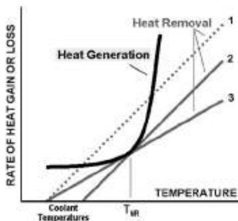
FIG. 23-16 For an exothermic reaction system with heat removal, e.g., to a vessel jacket and cooling coil, the limit of stable operation is reached as the reaction temperature increases to T_{NR} (temperature of no return), beyond which the rate of heat generation, which increases exponentially with increasing temperature, exceeds the capability of the system to remove the heat of reaction (see text).
