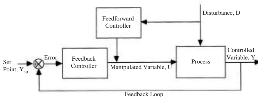
FIG. 8-1 Block diagram for feedforward and feedback control.
