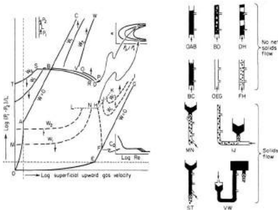
FIG. 17-2 Schematic phase diagram in the region of upward gas flow. W = mass flow solids, lb/(h \cdot ft^2) ; \epsilon = fraction voids; \rho_p = particle density, lb/ft^3 ; \rho_f = fluid density, lb/ft^3 ; C_D = drag coefficient; Re = modified Reynolds number. (Zenz and Othmer, Fluidization and Fluid Particle Systems , Reinhold, New York, 1960.)
