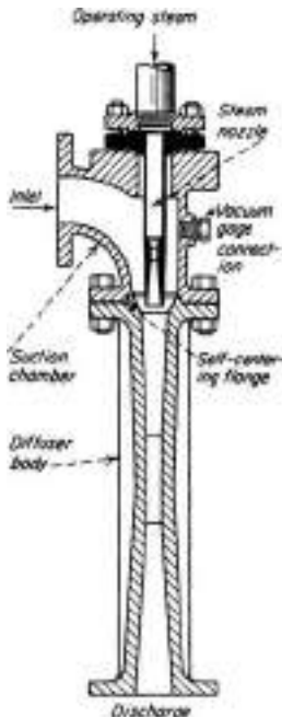
FIG. 10-98 Typical steam-jet ejector.
