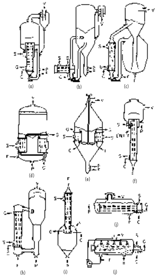
FIG. 11-122 Evaporator types. (a) Forced circulation. (b) Submerged-tube forced circulation. (c) Oslo-type crystallizer. (d) Short-tube vertical. (e) Propeller calandria. (f) Long-tube vertical. (g) Recirculating long-tube vertical. (h) Falling film. (i, j) Horizontal-tube evaporators. C = condensate; F = feed; G = vent; P = product; S = steam; V = vapor; ENT'T = separated entrainment outlet.
