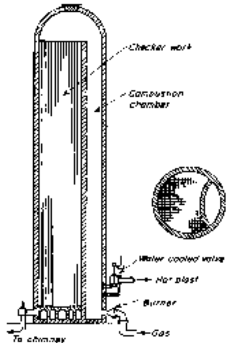
FIG. 24-61 Blast-furnace stove.
