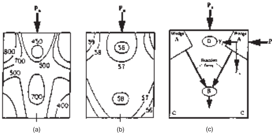
FIG. 21-139 Reaction in compacts of magnesium carbonate when pressed ( P_c = 671 \text{ kg/cm}^2 ). (a) Stress contour levels in kilograms per square centimeter. (b) Density contours in percent solids. (c) Reaction force developed at wedge responsible for stress and density patterns. [Train, Trans. Inst. Chem. Eng. (London), 35, 258 (1957).]
