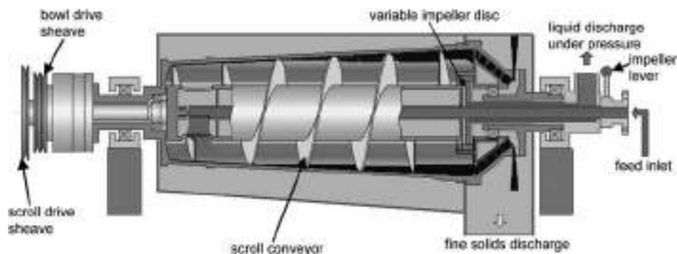
FIG. 18-159 Sedicanter centrifuge. (Flottweg Separation Technology.)
