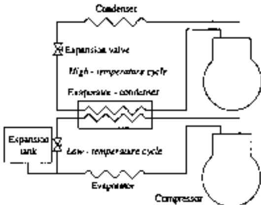
FIG. 11-80 Cascade system.
