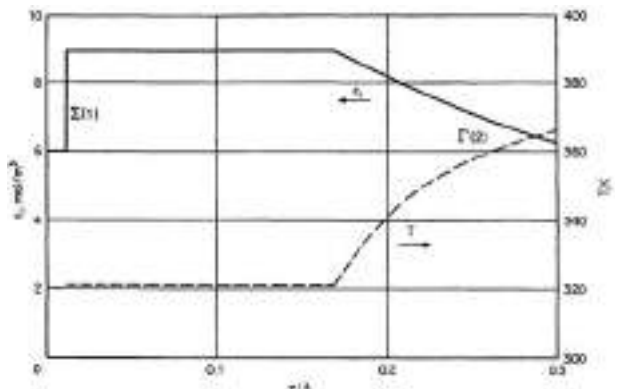
FIG. 16-25 Breakthrough curves for thermal regeneration.
