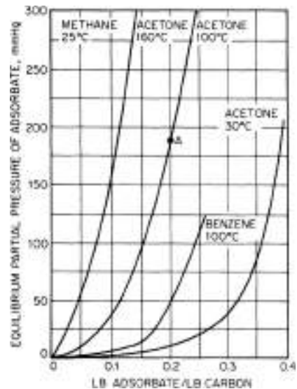
FIG. 22-9 Equilibrium partial pressures for certain organics on carbon.
