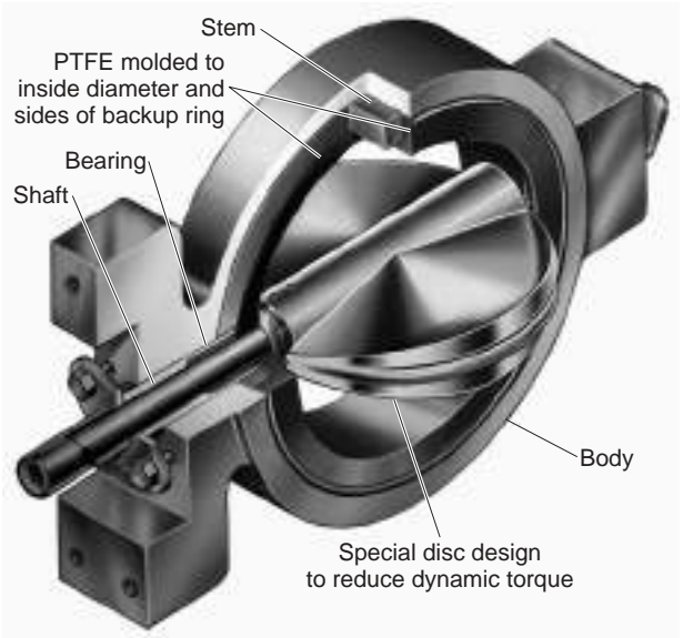
FIG. 8-68 Partial cutaway of wafer-style lined butterfly valve. (Courtesy Fisher Controls International LLC.)
