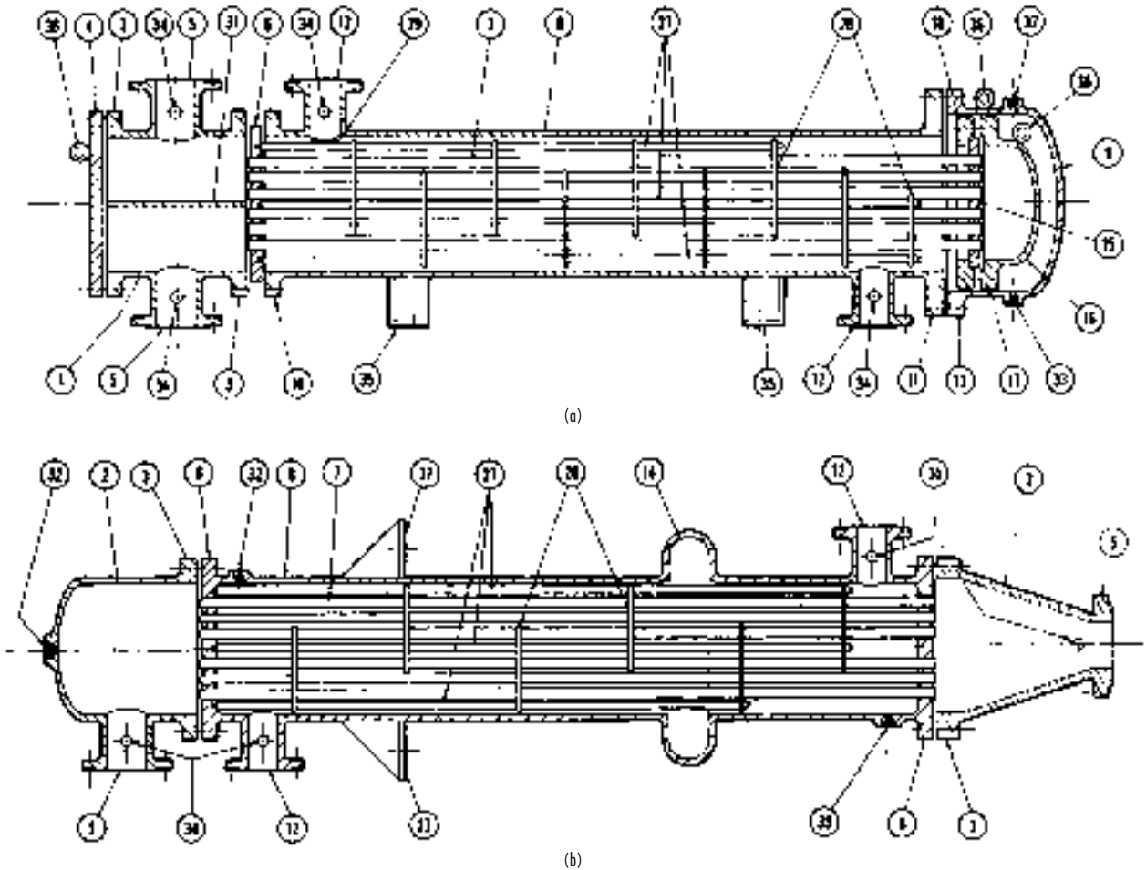
FIG. 11-36 Heat-exchanger-component nomenclature. (a) Internal-floating-head exchanger (with floating-head backing device). Type AES. (b) Fixed-tube-sheet exchanger. Type BEM. (Standards of the Tubular Exchanger Manufacturers Association, 6th ed., 1978.)
