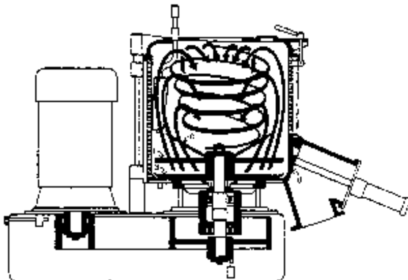
FIG. 18-52 High-intensity mixer: (a) bottom scraper; (b) fluidizing tool; (c) horn tool; (d) flush-mounted discharge valve. (Henschel Mixers America, Inc.)
