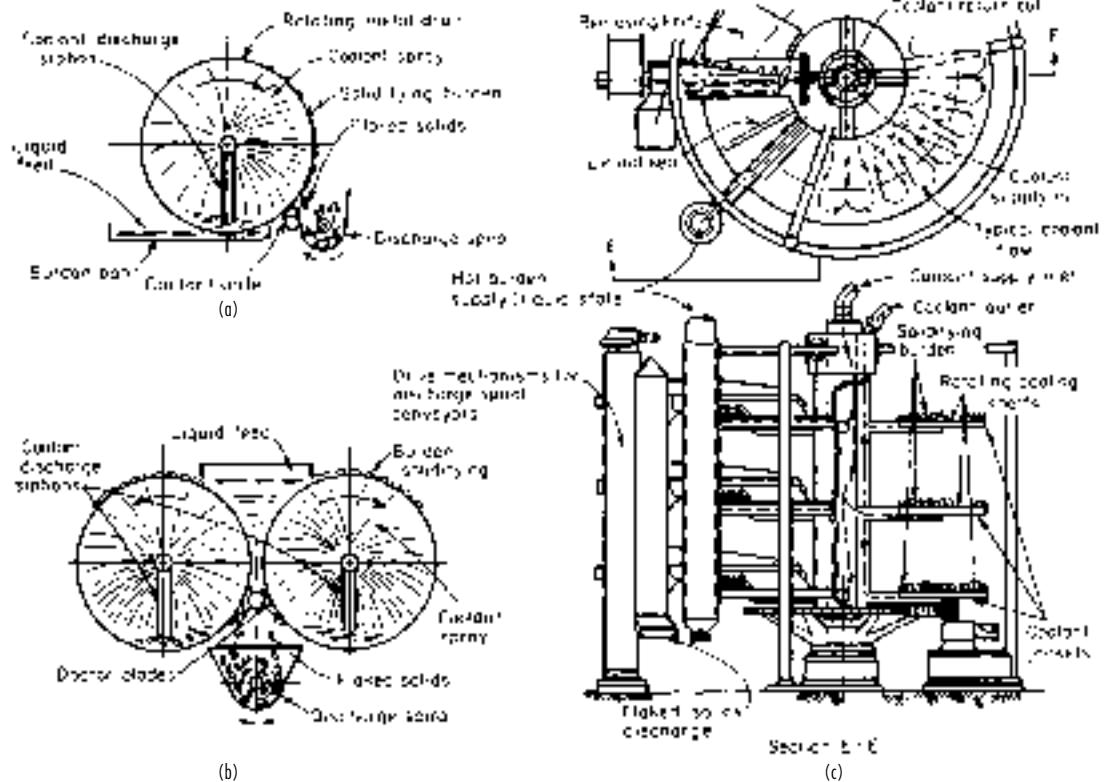
FIG. 11-55 Heat-transfer equipment for continuous solidification. (a) Single drum. (b) Twin drum. (c) Roto-shelf. (Courtesy of Buflovac Division, Blaw-Knox Food & Chemical Equipment, Inc.)
