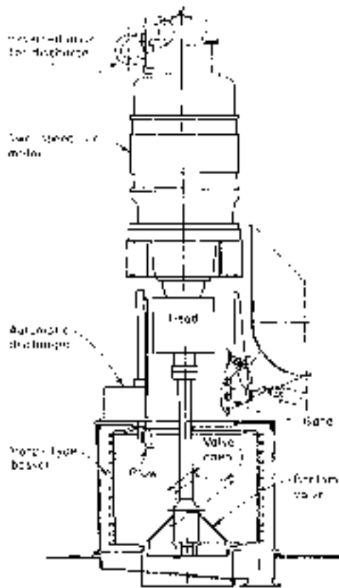
FIG. 18-165 Top-suspended vertical centrifuge. (Western States Machine Co.)
