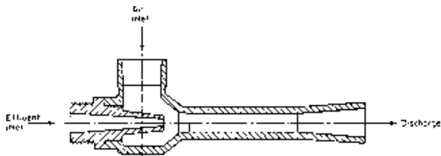
FIG. 14-100 Aeration ejector. (Penberthy, a division of Houdaille Industries, Inc.)
