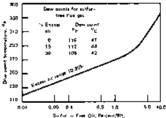
FIG. 24-21 Maximum flue-gas dew point versus percent of sulfur in typical oil fuels. (K = [°F + 459.7]/1.8)
