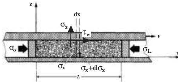
FIG. 21-144 Powder compaction in a channel, and associated force balance.
