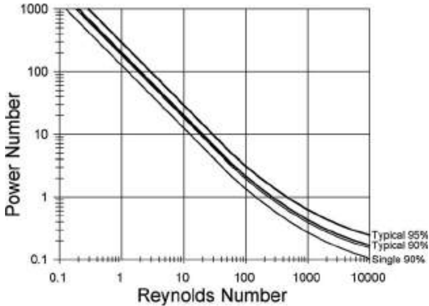
FIG. 18-45 Power numbers for helical-ribbon impeller: typical double-flight helices 95 percent of tank diameter T and 90 percent of T ; single-flight helix 90 percent of T ; single-flight 95 percent of T similar to double-flight 90 percent of T .
