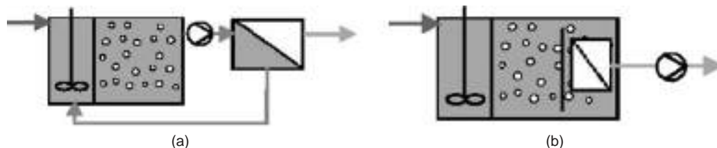
FIG. 22-45 Membrane bioreactor configurations for wastewater treatment. (a) With sidestream module; (b) with submerged module.
