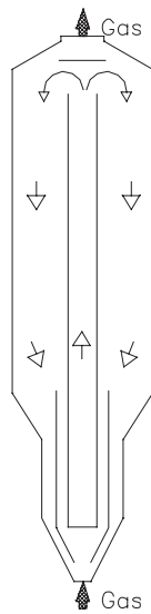
pneumatic granules mixer
