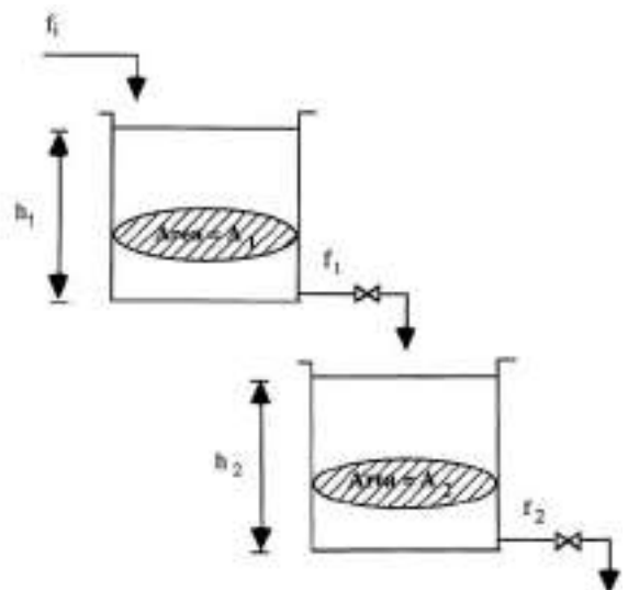
FIG. 8-12 Two tanks in series.
