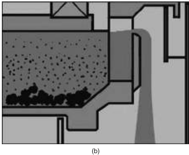
FIG. 18-156 (a) Section A from Fig. 18-155. (b) Detail B from Fig. 18-155. (Flottweg Separation Technology.)
