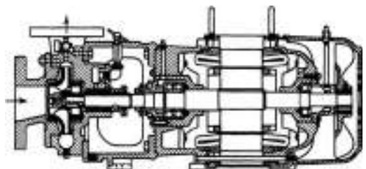
FIG. 10-49 Close-coupled pump.
