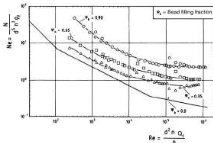
FIG. 20-77 Newton number as a function of Reynolds number for a horizontal stirred bead mill, with fluid alone and with various filling fractions of 1-mm glass beads [Weit and Schwedes, Chemical Engineering and Technology , 10 (6), 398–404 (1987)]. ( N = power input, W ; d = stirrer disk diameter, n = stirring speed, 1/s ; \mu = liquid viscosity, \text{Pa}\cdot\text{s} ; Q_f = feed rate, \text{m}^3/\text{s} .)
