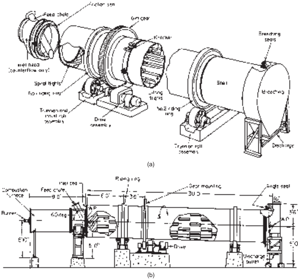
FIG. 12-58 Component arrangement (a) and elevation (b) of countercurrent direct-heat rotary dryer. (Air Preheater Company, Raymond® & Bartlett Snow™ Products.)
