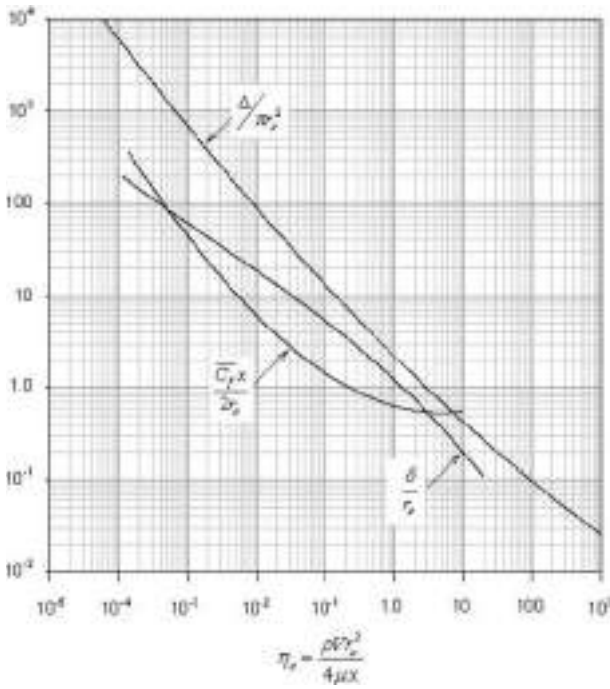
FIG 6-49 Boundary layer parameters for continuous cylindrical surfaces. ( \Delta/\pi r_o^2 is from Sakiadis, Am. Inst. Chem. Engr. J. , 7 , 467 [1961]; C_D x/2r_o , and \delta/r_o are from Vasudevan and Middleman, Am. Inst. Chem. Eng. J. , 16 , 614 [1970].)
