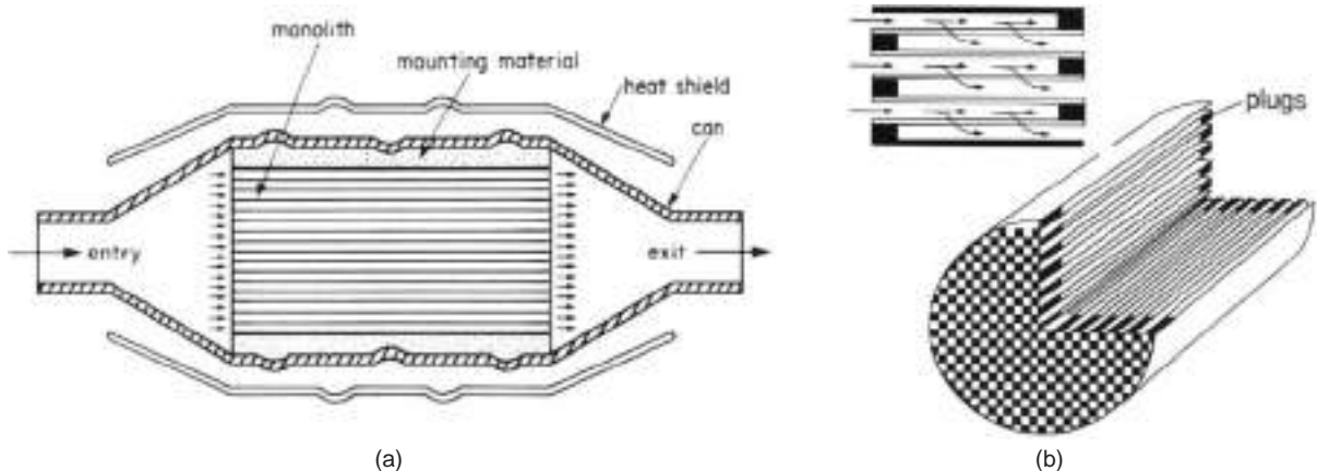
FIG. 19-18 Monolith catalysts. (a) Schematic of an automobile catalytic converter for the three-way removal of \text{CO} , hydrocarbons, and \text{NO}_x . (b) Schematic of a diesel trap. (Figs. 7.10 and 9.6 in Heck, Farrauto, and Gulati, Catalytic Air Pollution Control: Commercial Technology , Wiley-Interscience, 2002.)
