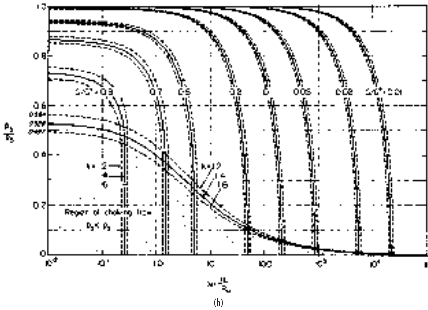
FIG. 6-21 Design charts for adiabatic flow of gases; (a) useful for finding the allowable pipe length for given flow rate; (b) useful for finding the discharge rate in a given piping system. (From Levenspiel, Am. Inst. Chem. Eng. J. , 23, 402 [1977].)
