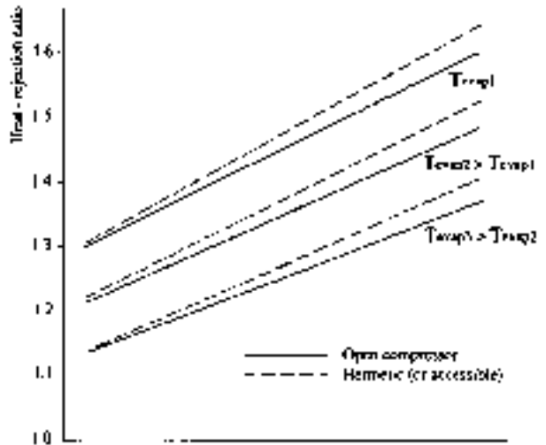
FIG. 11-89 Typical values of the heat-rejection ratio of the heat rejected at the condenser to the refrigeration capacity.
