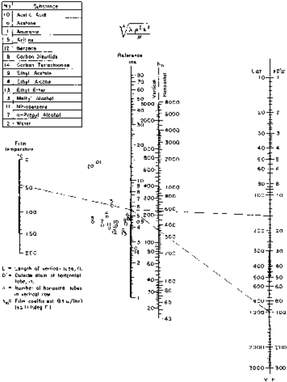
FIG. 5-7 Chart for determining heat-transfer coefficient h_m for film-type condensation of pure vapor, based on Eqs. (5-79) and (5-83). For vertical tubes multiply h_m by 1.2. If 4\Gamma/\mu exceeds 2100, use Fig. 5-8. \sqrt{\lambda\rho^2g/\mu} is in U.S. Customary units; to convert feet to meters, multiply by 0.3048; to convert inches to centimeters, multiply by 2.54; and to convert British thermal units per hour-square foot-degrees Fahrenheit to watts per square meter-kelvins, multiply by 5.6780.
