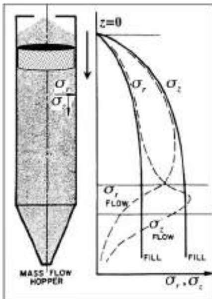
FIG. 21-40 Stresses in a vertical cylinder. [From Measuring Powder Flowability and Its Applications , E&G Associates, 2006, with permission.]
