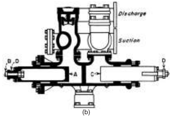
FIG. 10-27 Duplex single-acting plunger pump.
