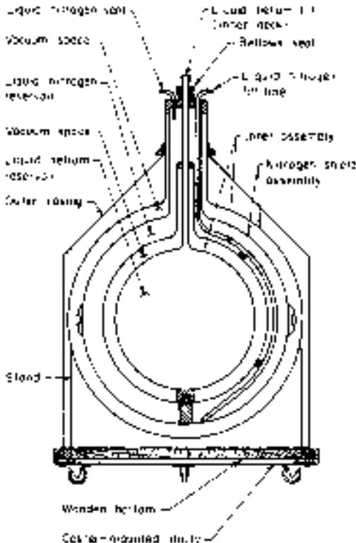
FIG. 11-67 Hydrogen bottle.
