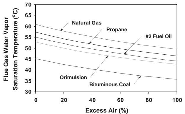
FIG. 24-57 Calculated flue gas water vapor dew points, for different fuel types, as a function of excess air [Orimulsion (28.3% water), Pittsburgh Seam 8 (5% water)]. (Courtesy T. A. Butcher, US DOE; www.bnl.gov .)
