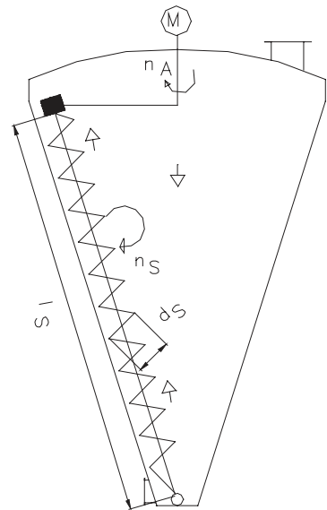
conical screw mixer
