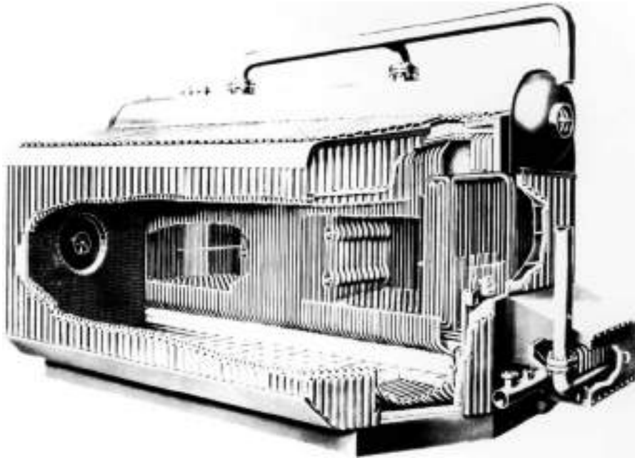
FIG. 24-40 A D-type shop-assembled water-tube boiler. (Combustion Engineering, Inc.)
