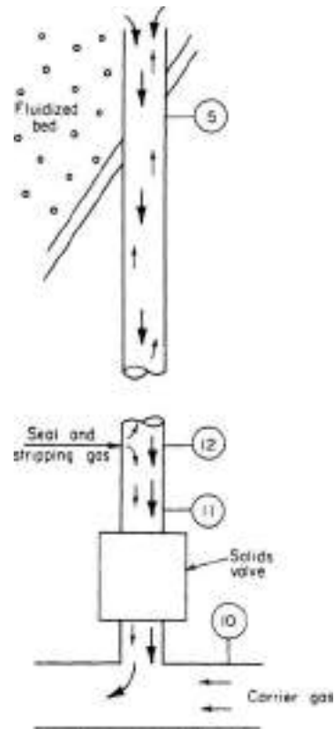
FIG. 17-20 Fluidized-bed seal leg.
