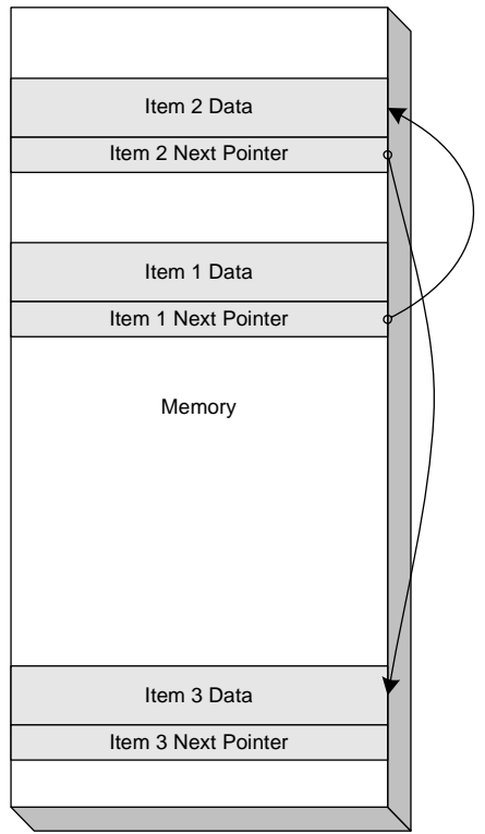
Figure C.2 Logical and in-memory arrangement of a singly linked list.
