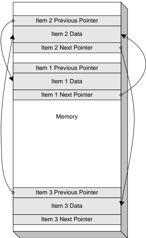
Figure C.3 Doubly linked list layout—logically and in memory.
